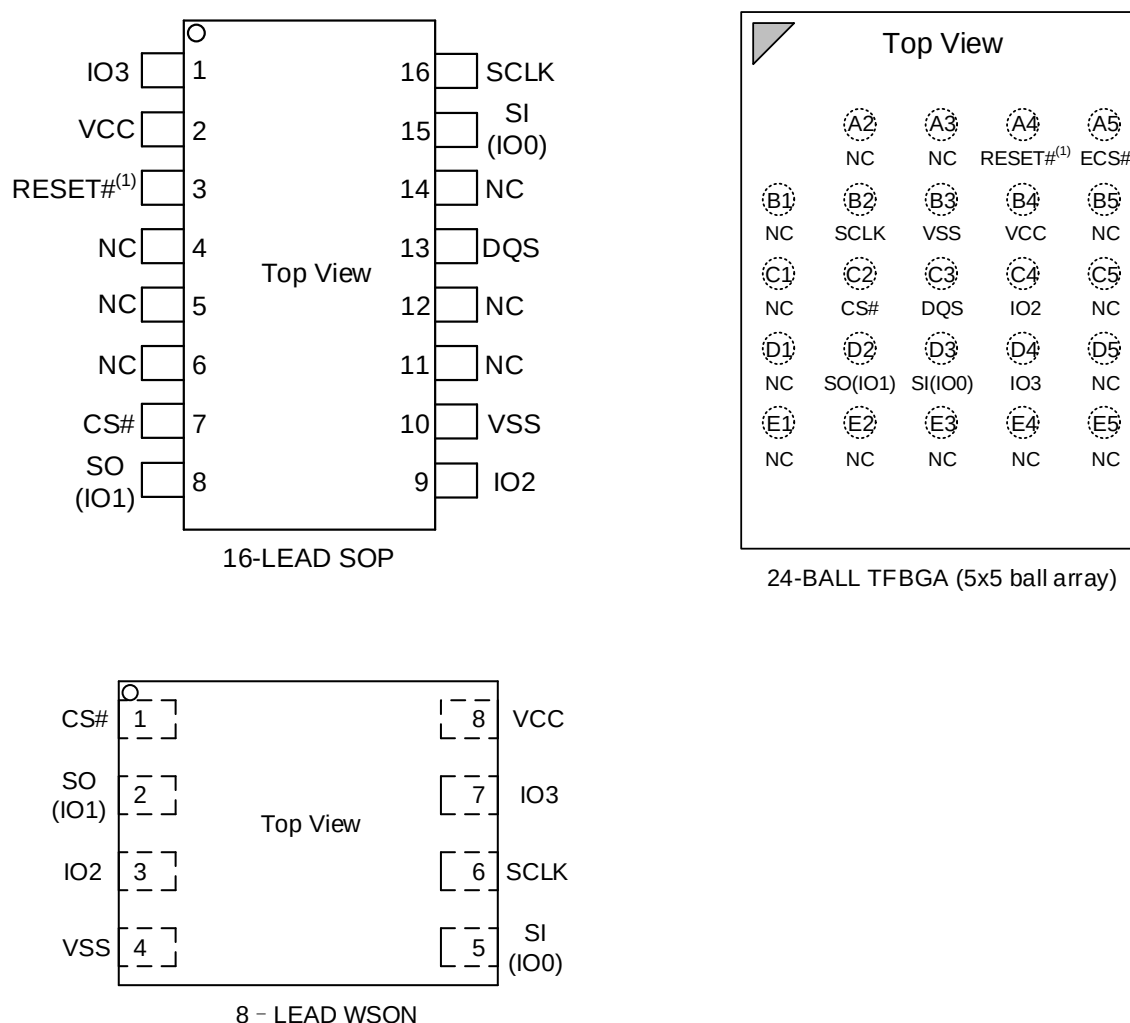
Figure 1. Connection Diagram
