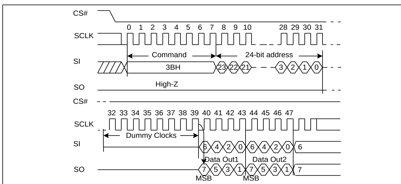
Figure 16. Dual Output Fast Read Sequence Diagram (ADS=0)
