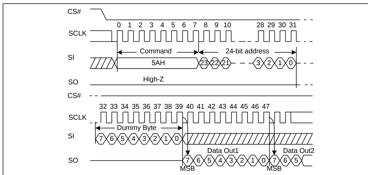
Figure 59. Read Serial Flash Discoverable Parameter command Sequence Diagram
