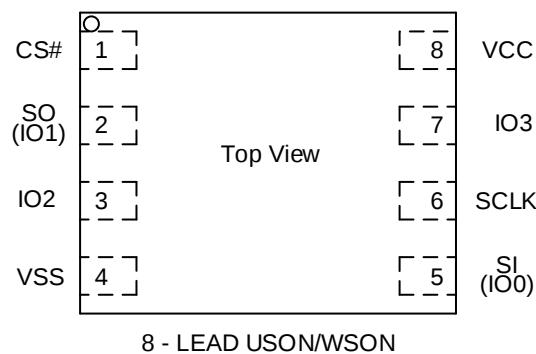
Figure 1 Connection Diagram for USON8/WSN8 package
