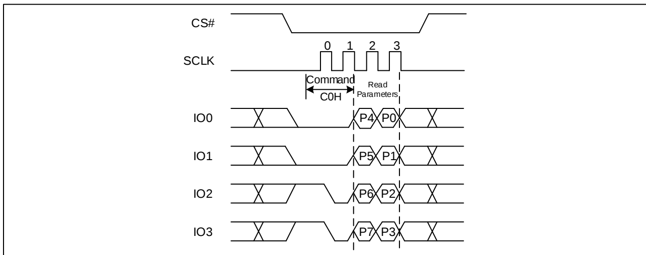
Figure 35. Set Read Parameters command Sequence Diagram
