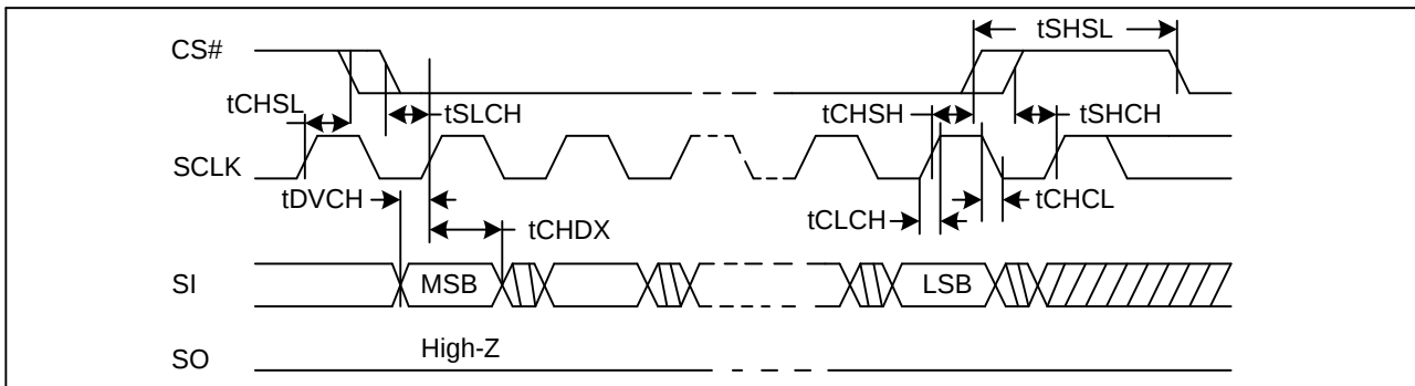
Figure 64. Input Timing
