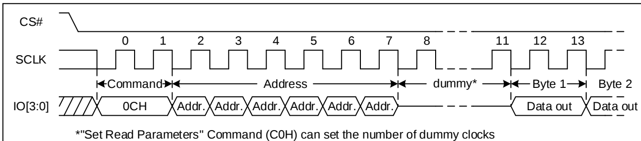
Figure 46. Burst Read with Wrap command Sequence Diagram
