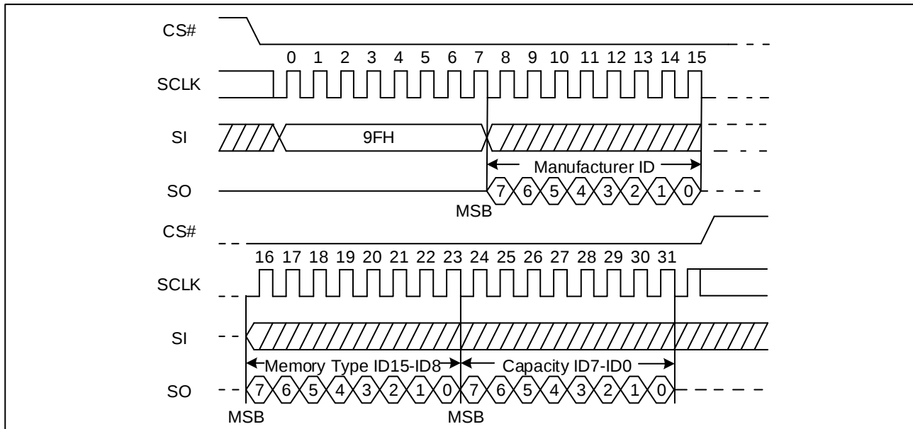
Figure 38. Read Identification ID Sequence Diagram (SPI)
