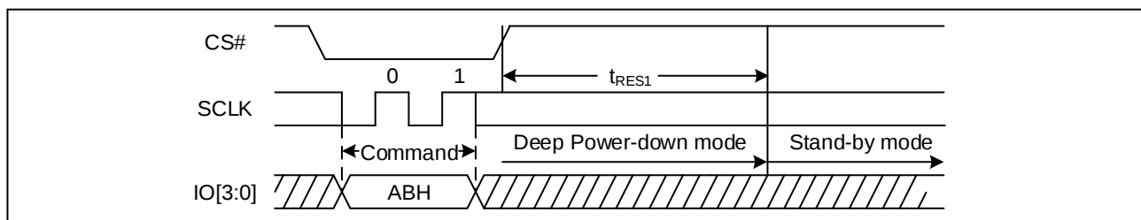
Figure 54. Release Power-Down Sequence Diagram (QPI)
