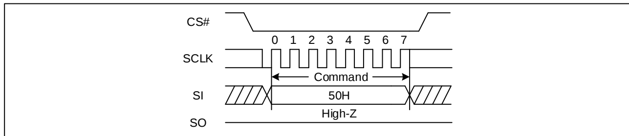
Figure 11. Write Enable for Volatile Status Register Sequence Diagram (SPI)
