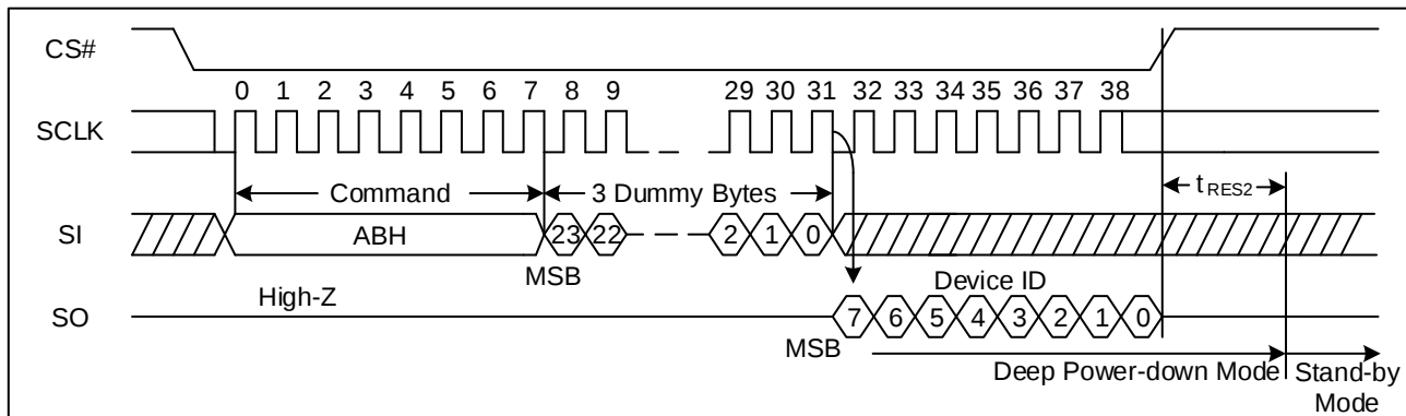
Figure 55. Release Power-Down/Read Device ID Sequence Diagram (SPI)
