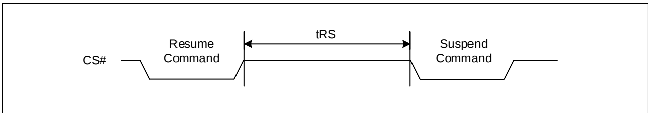
Figure 66. Resume to Suspend Timing Diagram
