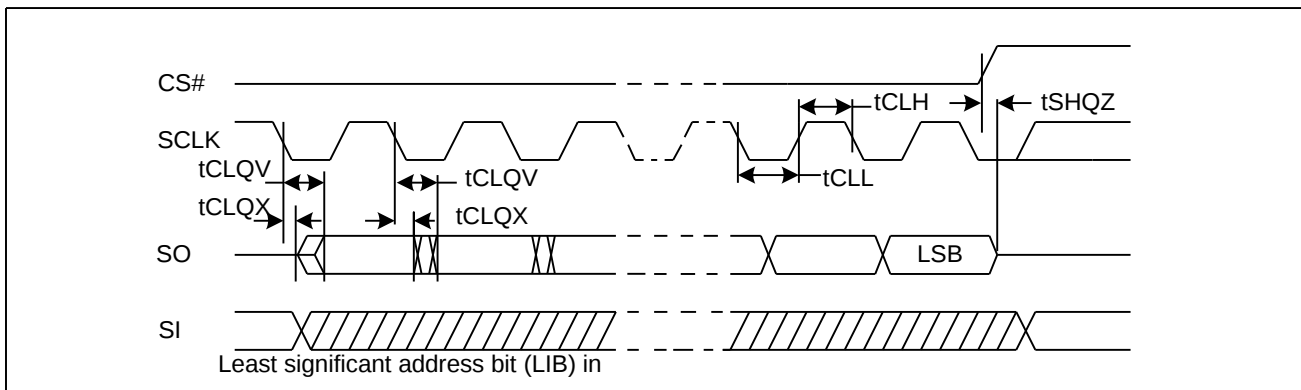
Figure 65. Output Timing
