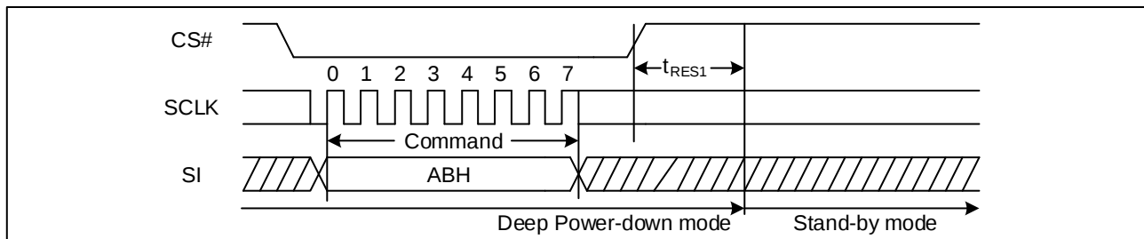
Figure 53. Release Power-Down Sequence Diagram (SPI)
