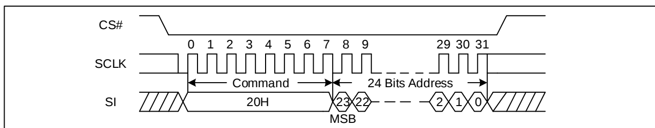
Figure 27. Sector Erase Sequence Diagram (SPI)
