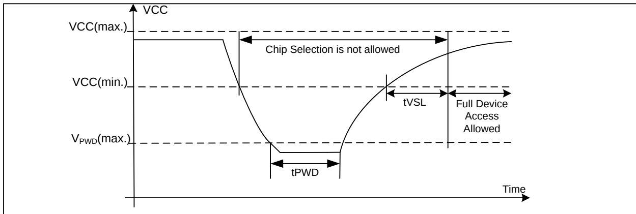
Figure 61. Power-On Timing Sequence Diagram
