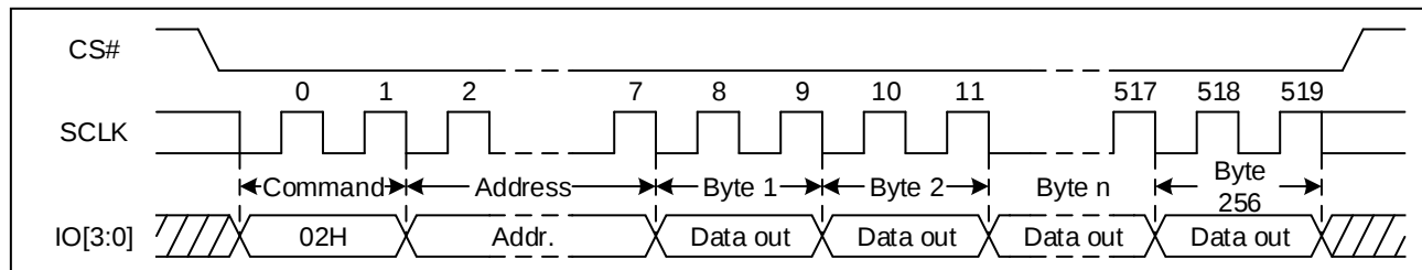
Figure 25. Page Program Sequence Diagram (QPI)
