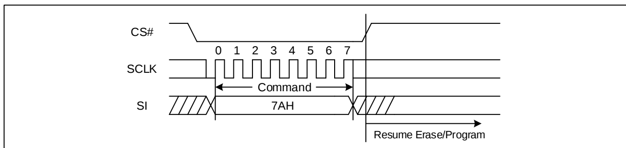
Figure 49. Program/Erase Resume Sequence Diagram (SPI)
