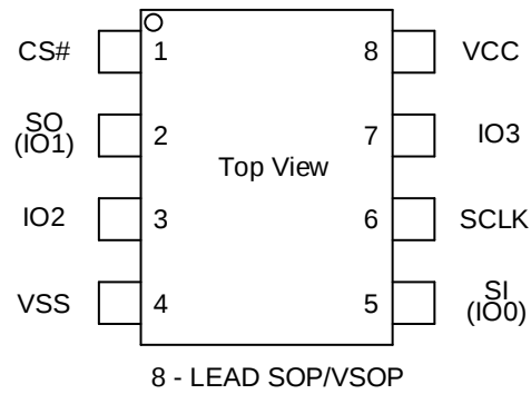
Figure 2 Connection Diagram for SOP8/VSOP8 package
