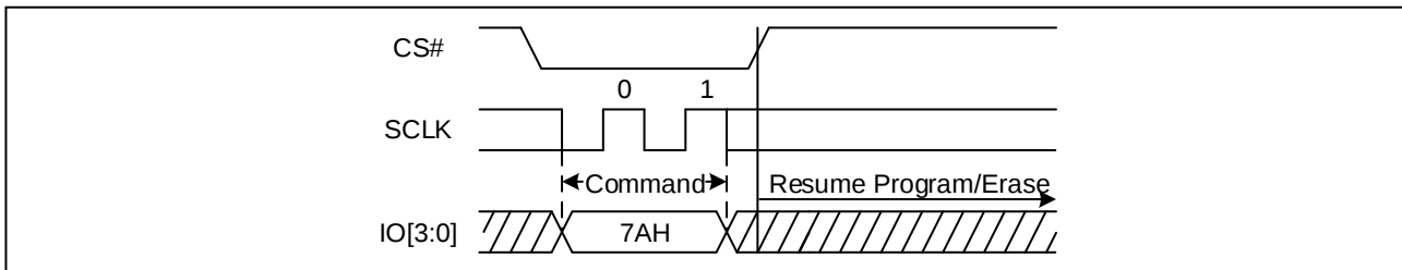
Figure 50. Program/Erase Resume Sequence Diagram (QPI)
