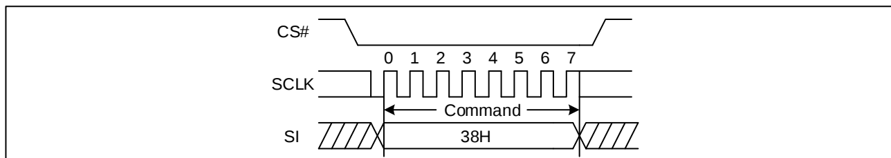
Figure 57. Enable QPI mode command Sequence Diagram
