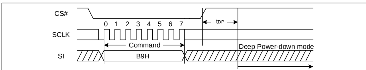
Figure 51. Deep Power-Down Sequence Diagram (SPI)
