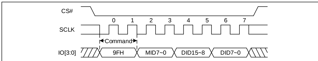
Figure 39. Read Identification ID Sequence Diagram (QPI)
