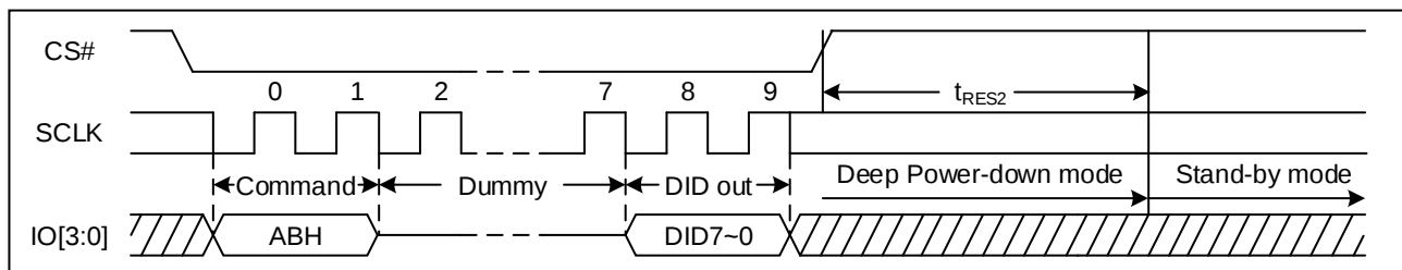
Figure 56. Release Power-Down/Read Device ID Sequence Diagram (QPI)
