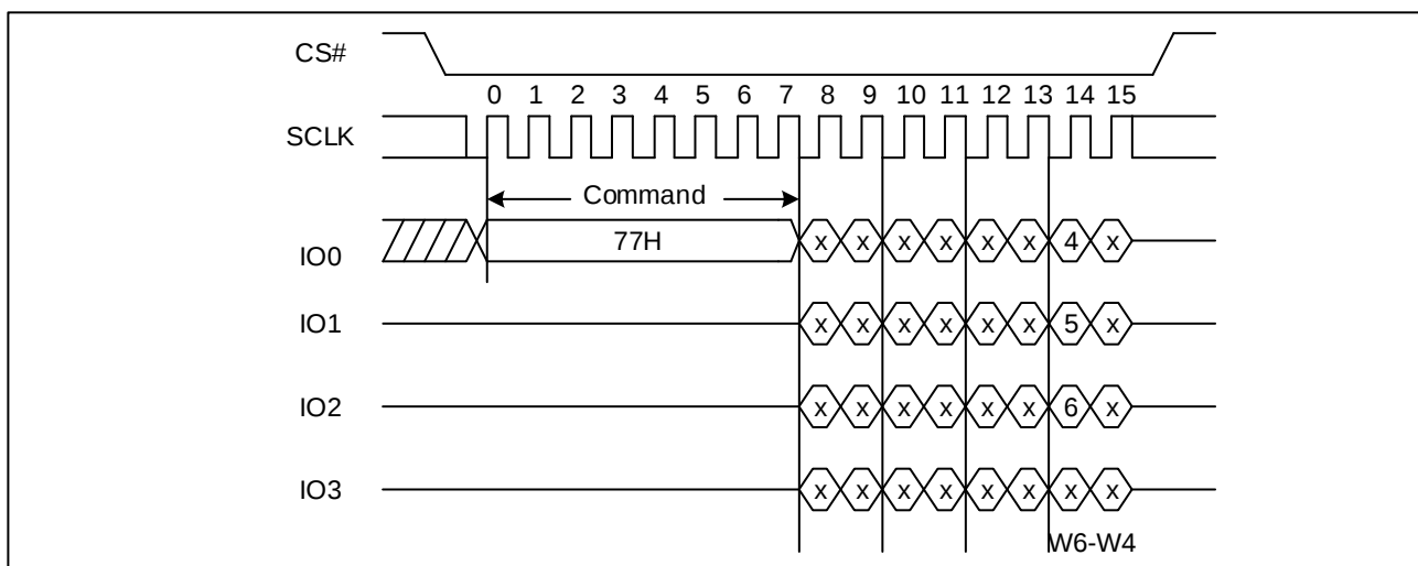
Figure 23. Set Burst with Wrap Sequence Diagram
