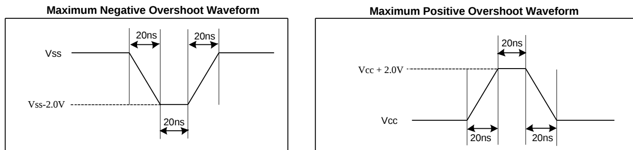
Figure 62. Input Test Waveform and Measurement Level
