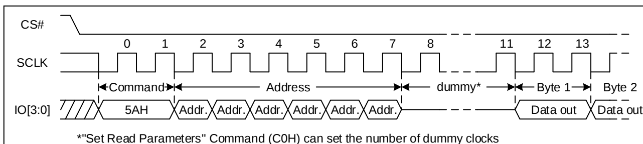
Figure 60. Read Serial Flash Discoverable Parameter command Sequence Diagram (QPI)
