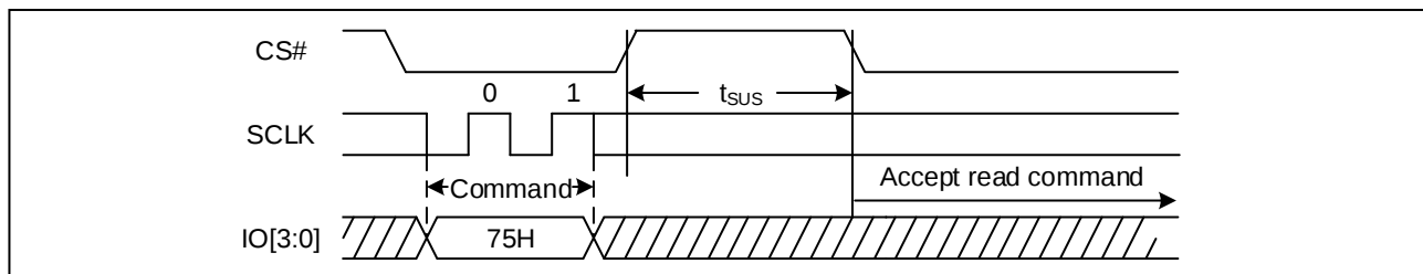
Figure 48. Program/Erase Suspend Sequence Diagram (QPI)
