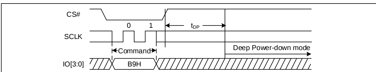
Figure 52. Deep Power-Down Sequence Diagram (QPI)
