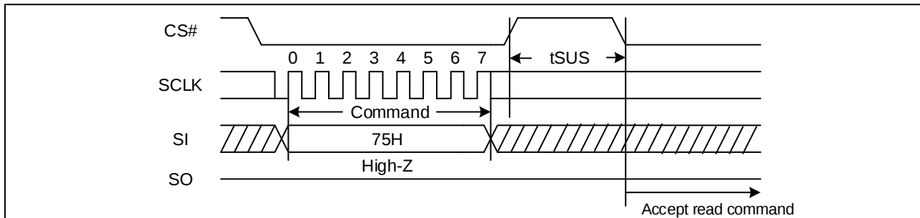
Figure 47. Program/Erase Suspend Sequence Diagram (SPI)
