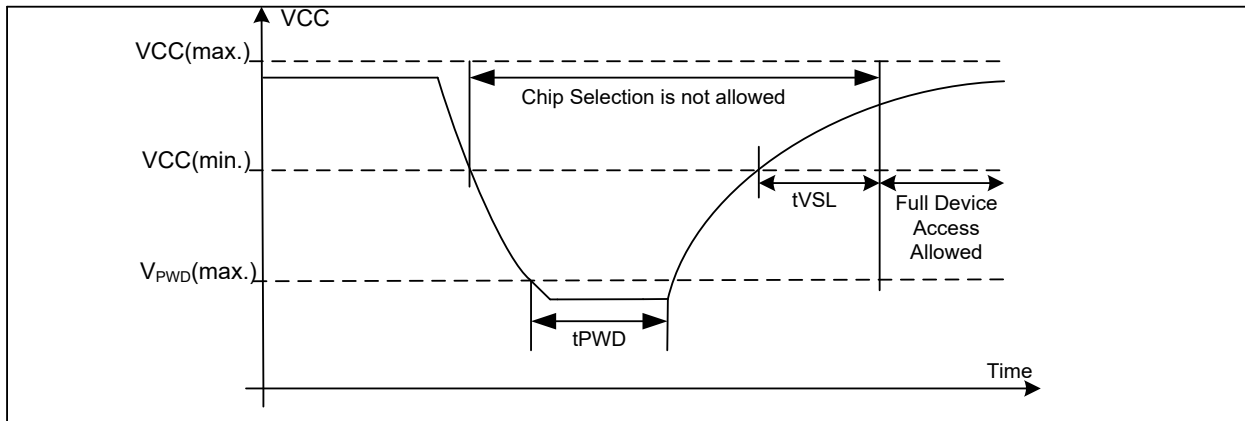
Figure 36. Power-Up/Down Timing Sequence Diagram
