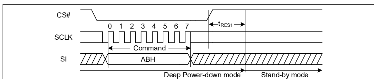
Figure 24. Release Power-Down Sequence Diagram
