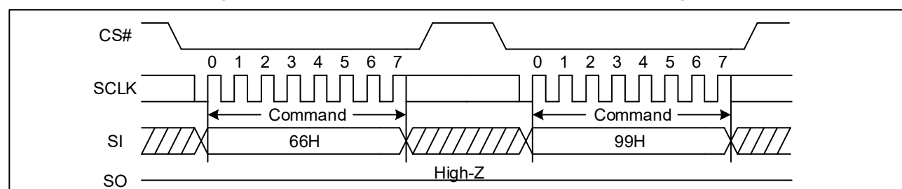
Figure 34. Enable Reset and Reset command Sequence Diagram
