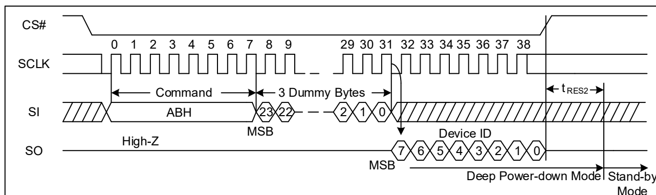
Figure 25. Release Power-Down/Read Device ID Sequence Diagram
