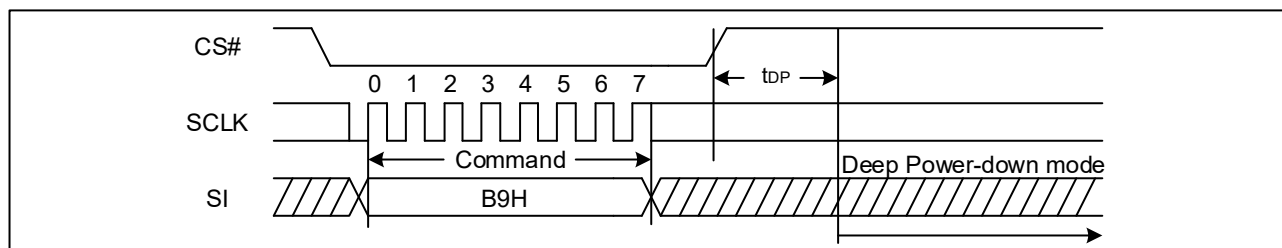
Figure 23. Deep Power-Down Sequence Diagram
