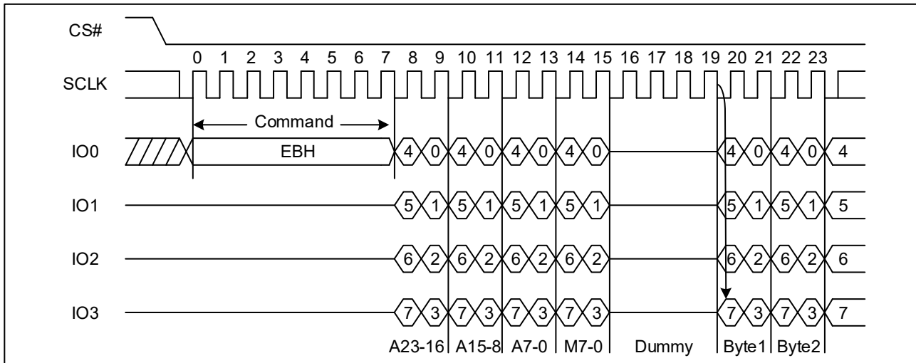
Figure 14. Quad I/O Fast Read Sequence Diagram ((M5-4) \neq (1, 0))
