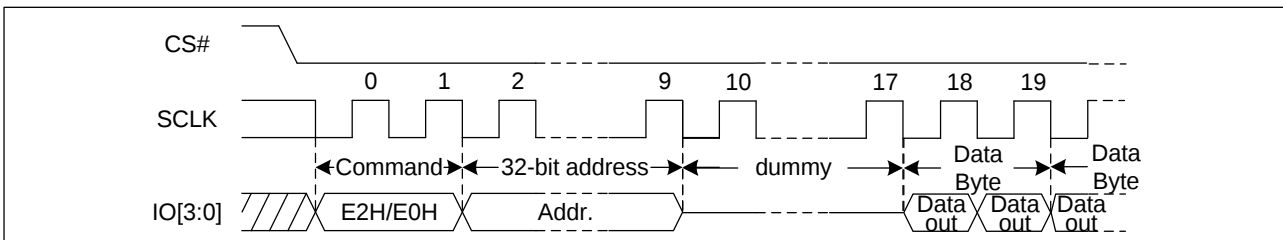
Figure 90 Read NL Register/VL Register Sequence (QPI)
