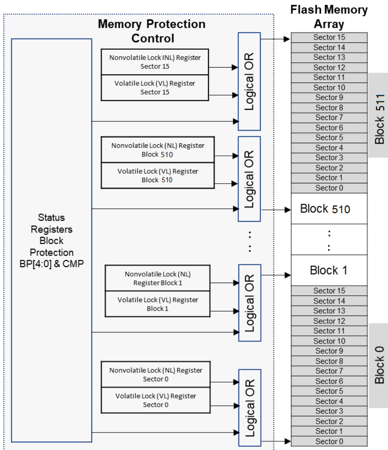
Figure 5 Memory Protection Control Overview
