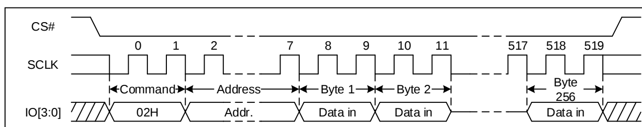
Figure 49 Page Program Sequence Diagram (QPI)
