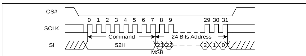
Figure 53 32KB Block Erase Sequence Diagram (SPI)
