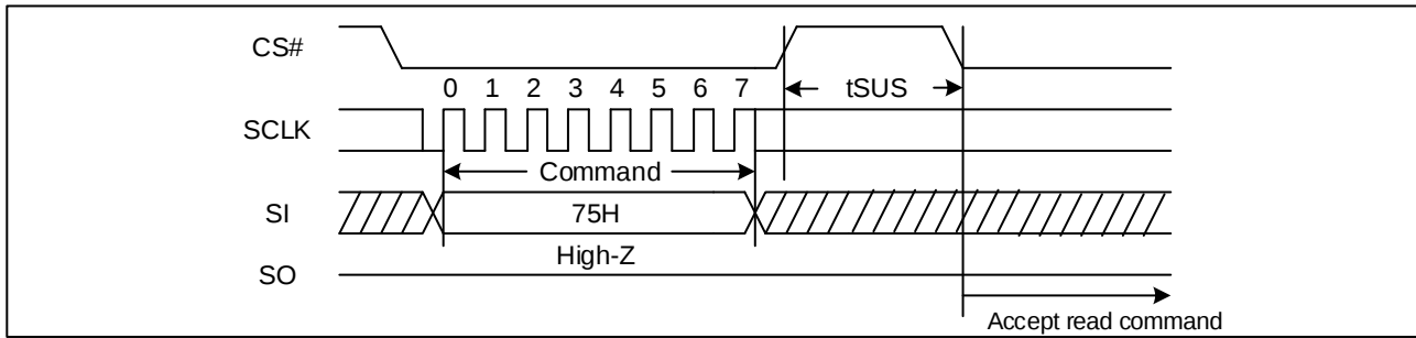
Figure 72 Program/Erase Suspend Sequence Diagram (SPI)
