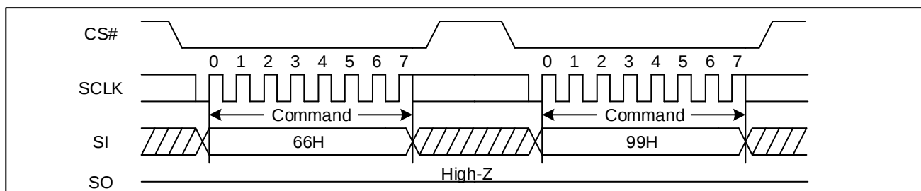
Figure 91 Enable Reset and Reset command Sequence Diagram (SPI)
