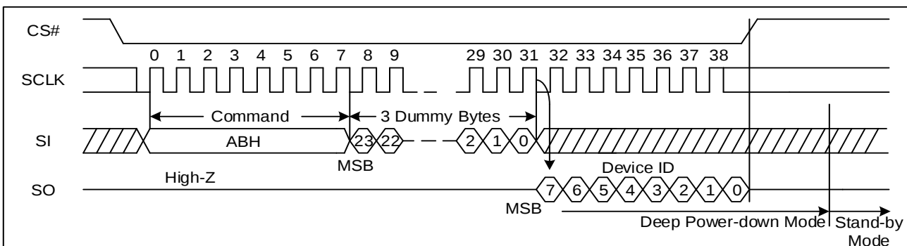
Figure 65. Release Power-Down/Read Device ID Sequence Diagram (SPI)
