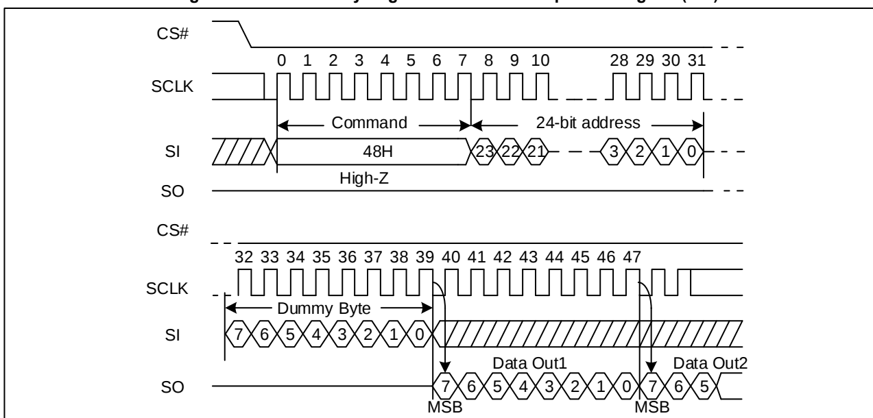
Figure 78 Read Security Registers command Sequence Diagram (SPI)
