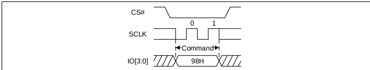
Figure 80 Global Block/Sector Unlock Sequence Diagram (QPI)
