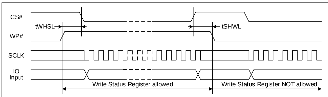
Figure 104. WP# Timing
