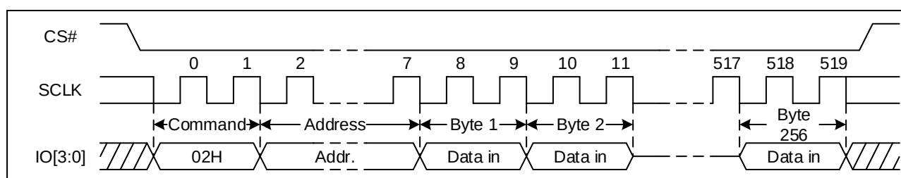
Figure 46 Page Program Sequence Diagram (QPI)
