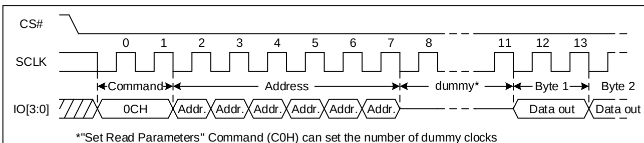
Figure 42. Burst Read with Wrap Sequence Diagram
