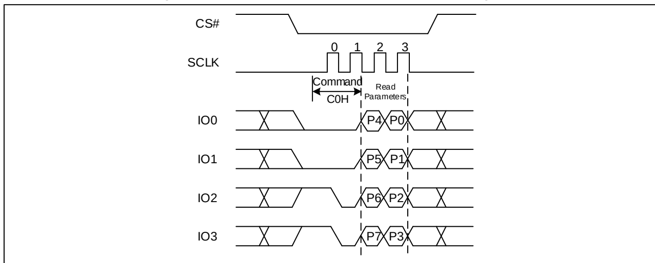
Figure 44. Set Read Parameters command Sequence Diagram
