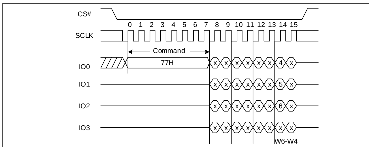
Figure 43. Set Burst with Wrap Sequence Diagram
