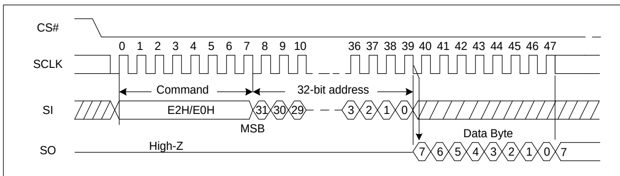
Figure 87 Read NL Register/VL Register Sequence Diagram (SPI)
