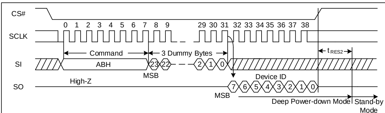
Figure 63. Release Power-Down/Read Device ID Sequence Diagram (SPI)
