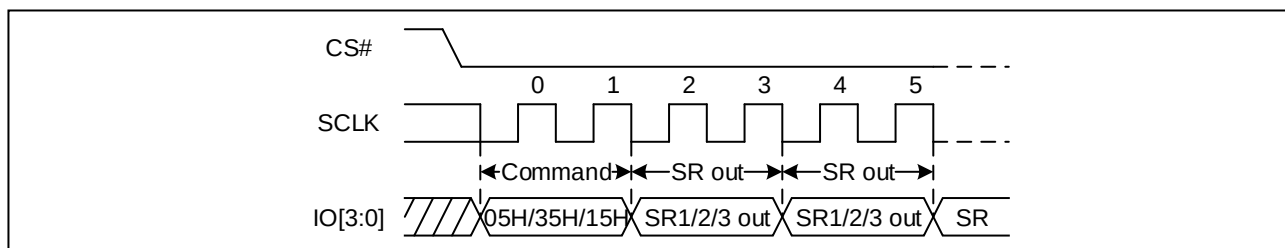
Figure 27 Read Status Register Sequence Diagram (QPI)
