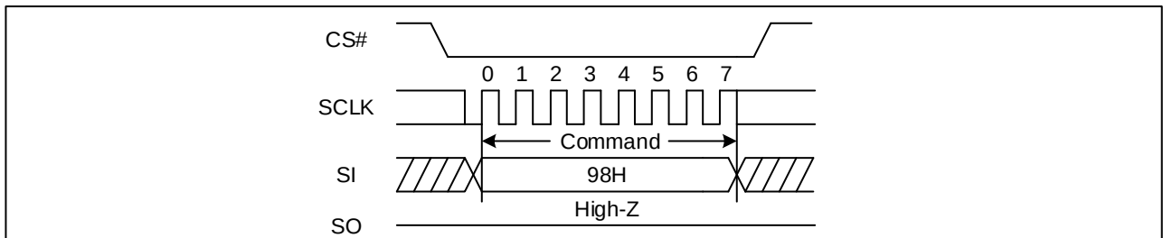
Figure 79 Global Block/Sector Unlock Sequence Diagram (SPI)
