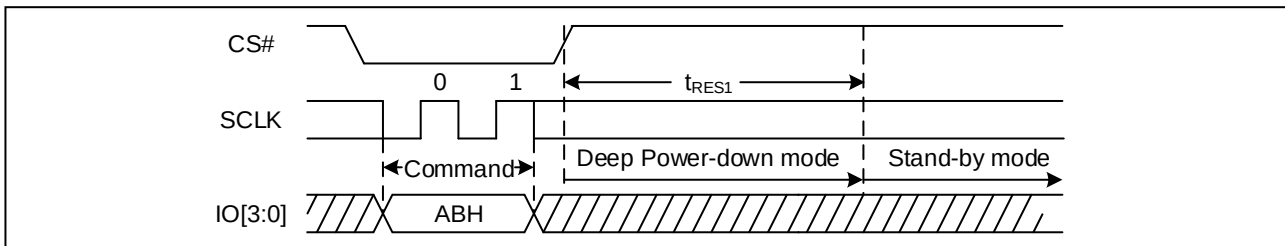
Figure 62 Release Power-Down Sequence Diagram (QPI)
