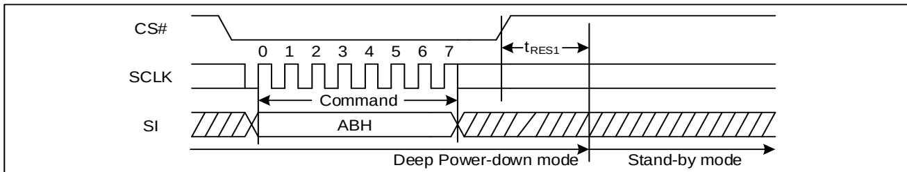
Figure 61 Release Power-Down Sequence Diagram (SPI)
