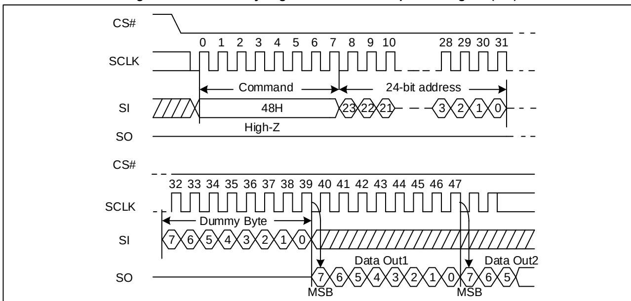
Figure 76 Read Security Registers command Sequence Diagram (SPI)
