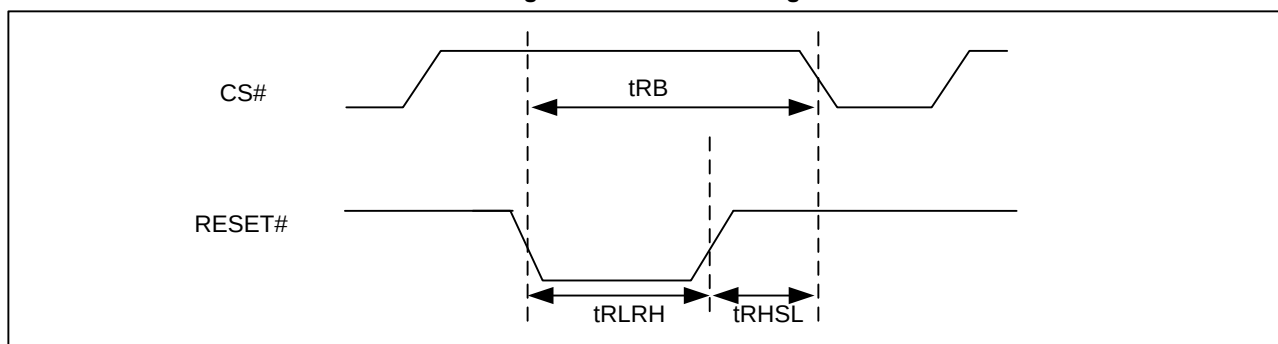
Figure 105. RESET Timing
