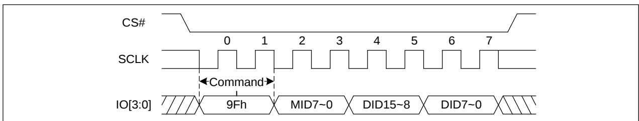
Figure 56. Read Identification ID Sequence Diagram (QPI)
