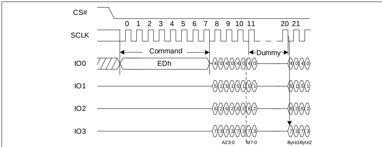
Figure 32. DTR Quad I/O Fast Read Sequence Diagram (SPI, (M5-4) ≠ (1, 0))
