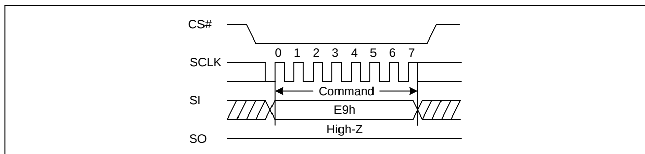
Figure 51 Disable 4-Byte Mode Sequence Diagram (SPI)
