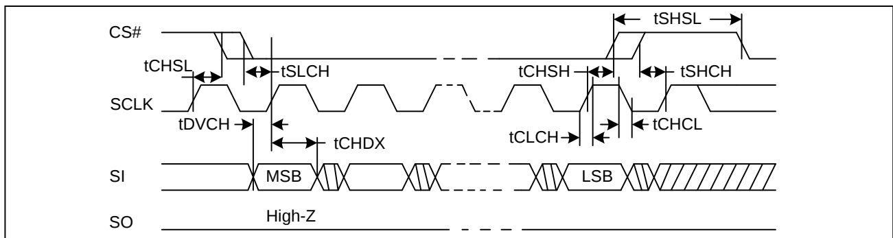
Figure 80. Input Timing
