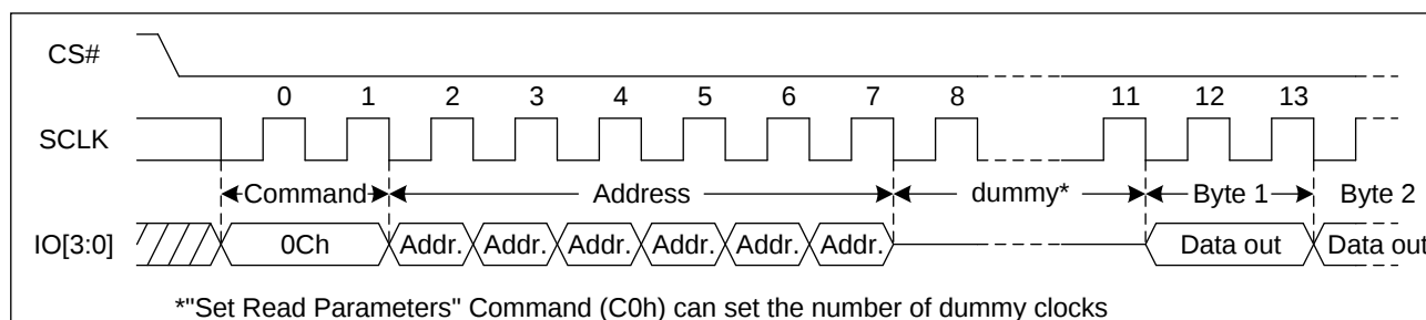
Figure 35. Burst Read with Wrap command Sequence Diagram
