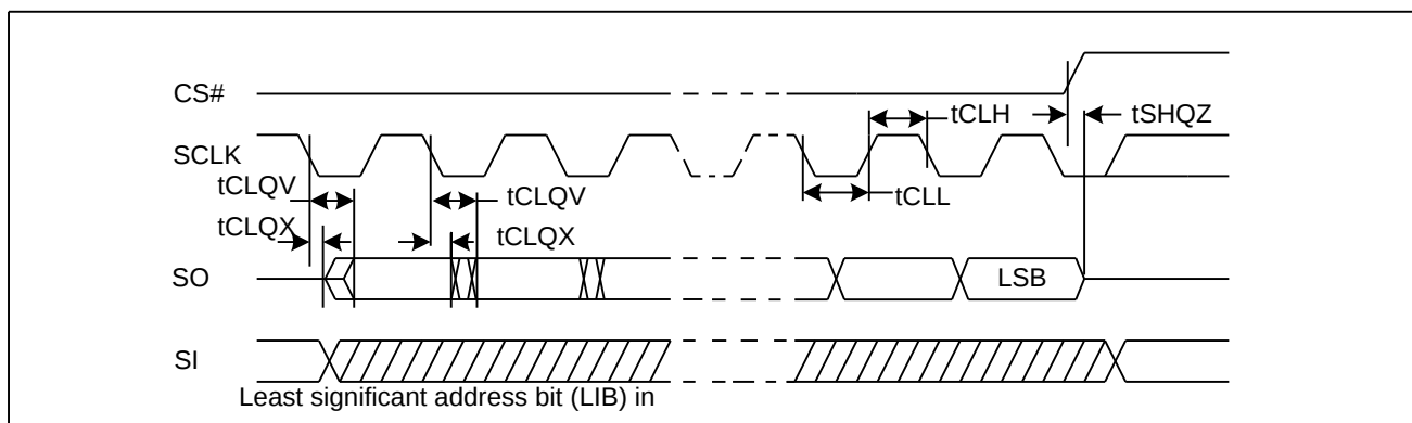
Figure 81. Output Timing
