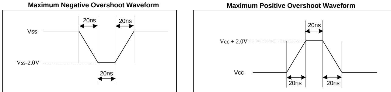
Figure 78. Input Test Waveform and Measurement Level
