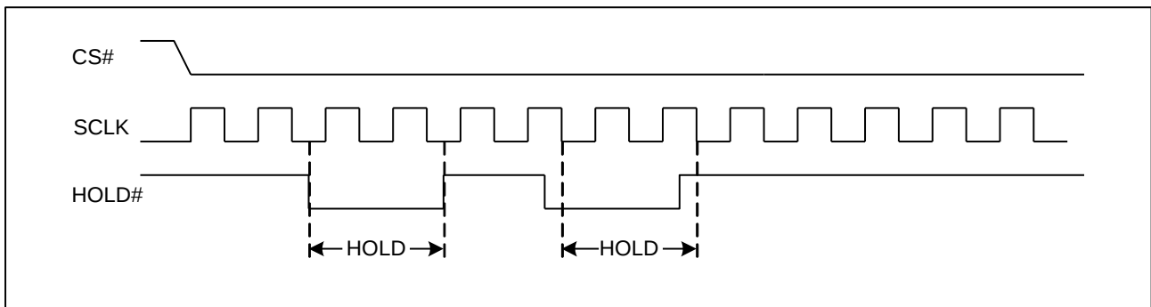
Figure 2 HOLD Condition
