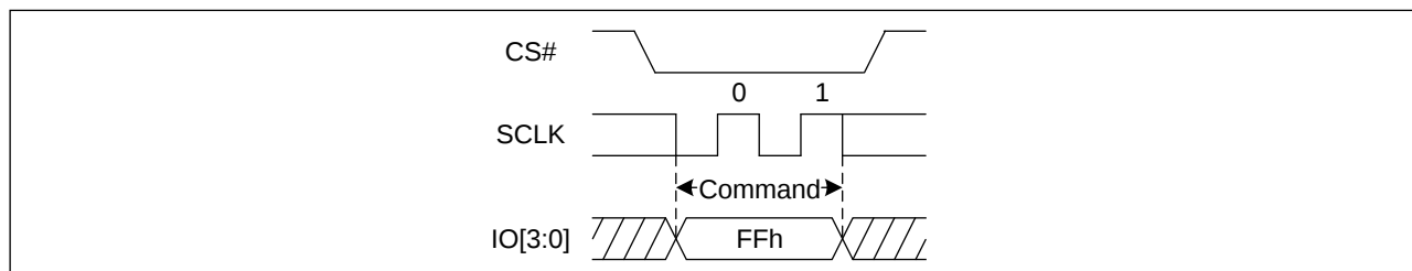
Figure 74. Disable QPI mode command Sequence Diagram
