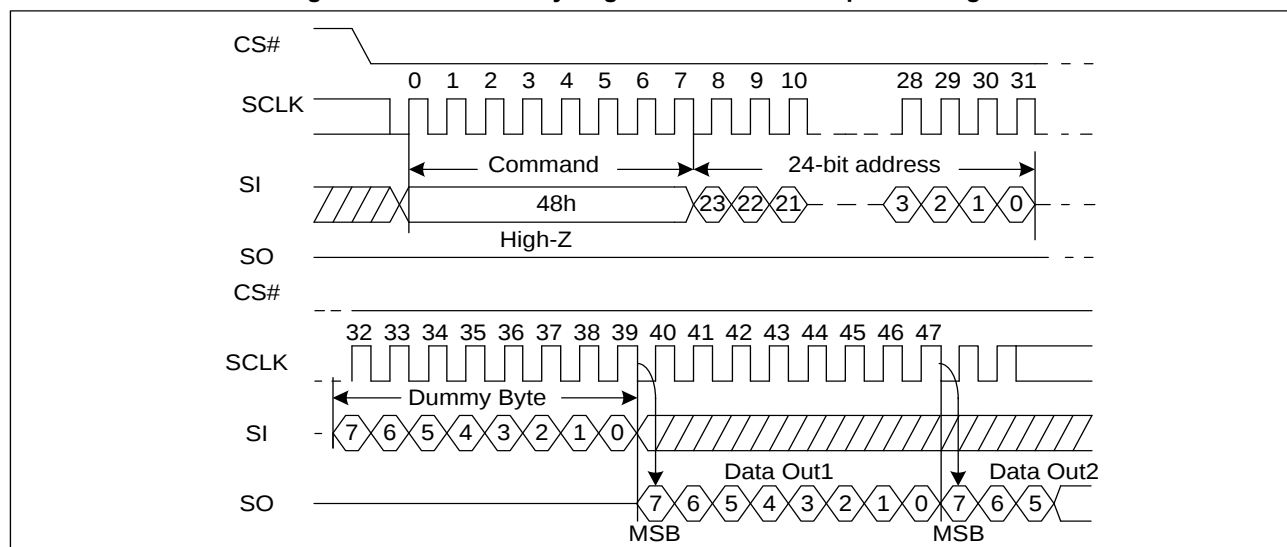
Figure 60. Read Security Registers command Sequence Diagram
