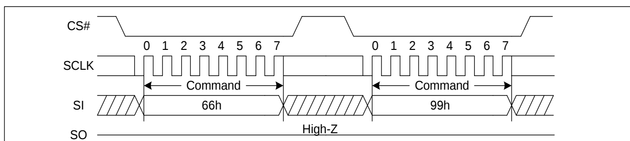
Figure 61. Enable Reset and Reset command Sequence Diagram (SPI)
