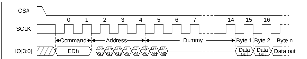
Figure 33. DTR Quad I/O Fast Read Sequence Diagram (QPI, (M5-4) ≠ (1, 0))
