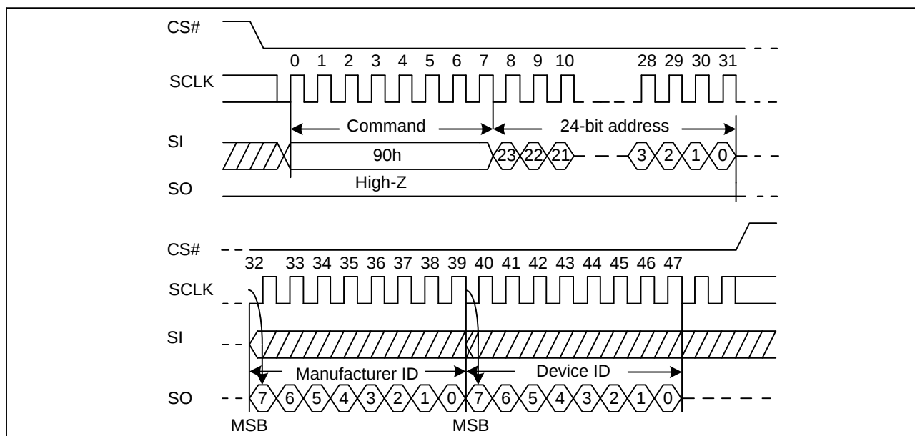
Figure 53. Read Manufacture ID/ Device ID Sequence Diagram (SPI)
