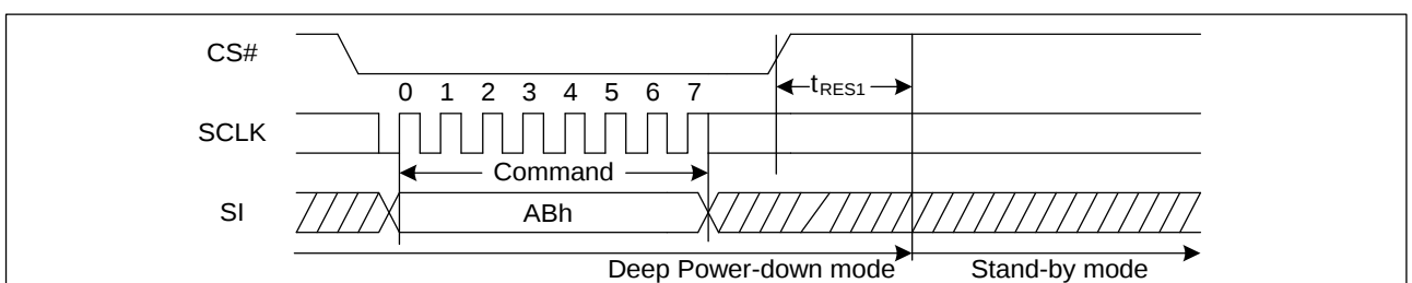
Figure 69. Release Power-Down Sequence Diagram (SPI)
