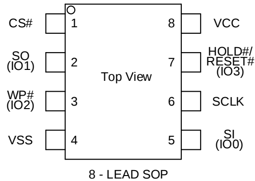
Figure 1 Connection Diagram for SOP8 package
