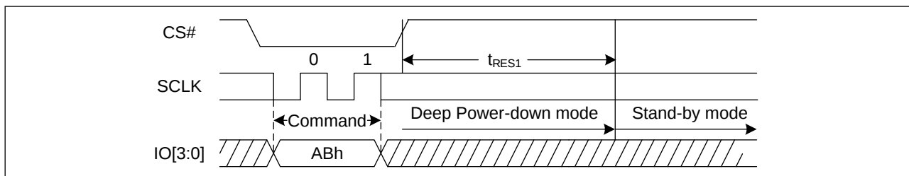
Figure 70. Release Power-Down Sequence Diagram (QPI)
