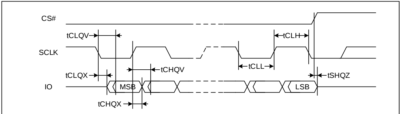
Figure 83. Serial Output Timing (DTR)
