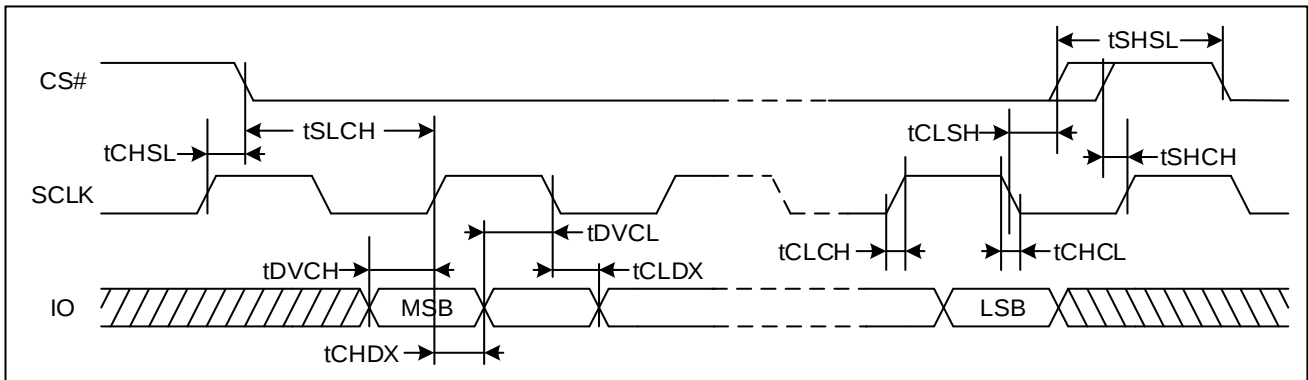
Figure 82. Serial Input Timing (DTR)
