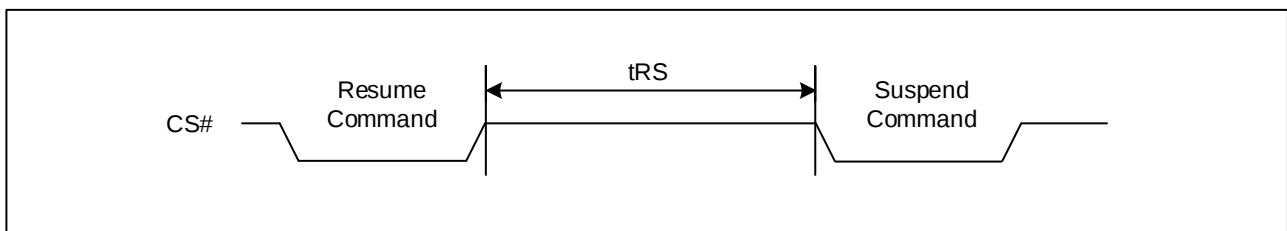
Figure 84. Resume to Suspend Timing Diagram
