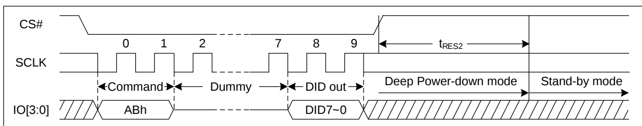
Figure 72. Release Power-Down/Read Device ID Sequence Diagram (QPI)
