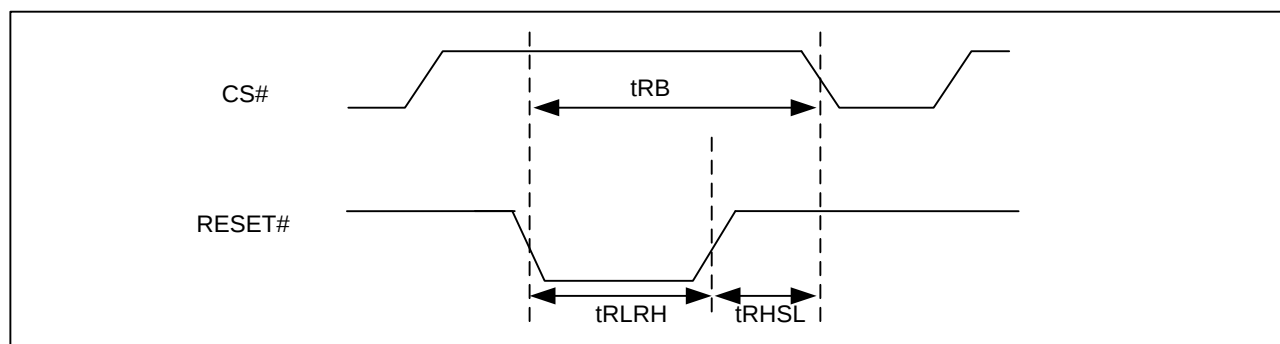
Figure 87 RESET# Timing
