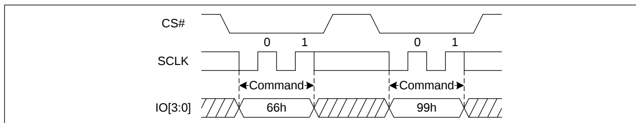
Figure 62. Enable Reset and Reset command Sequence Diagram (QPI)
