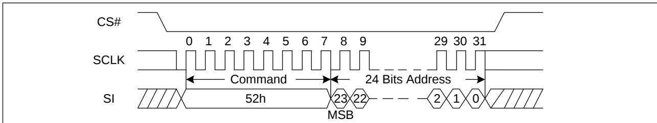
Figure 43. 32KB Block Erase Sequence Diagram (SPI)
