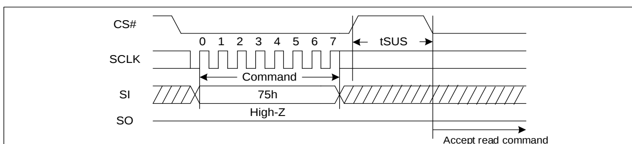
Figure 63. Program/Erase Suspend Sequence Diagram (SPI)
