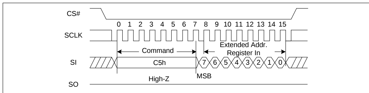
Figure 16. Write Extended Address Register Sequence Diagram (SPI)
