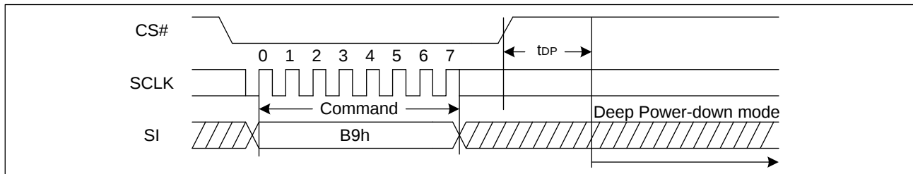
Figure 67. Deep Power-Down Sequence Diagram (SPI)
