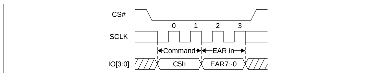
Figure 17. Write Extended Address Register Sequence Diagram (QPI)
