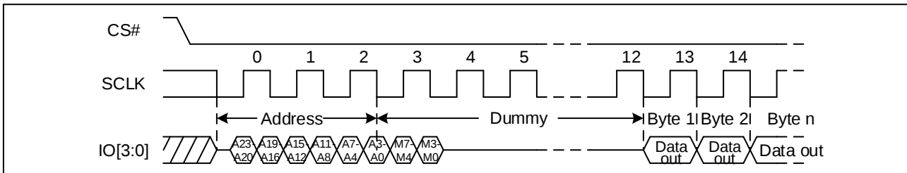
Figure 34. DTR Quad I/O Fast Read Sequence Diagram ((M5-4) = (1, 0))
