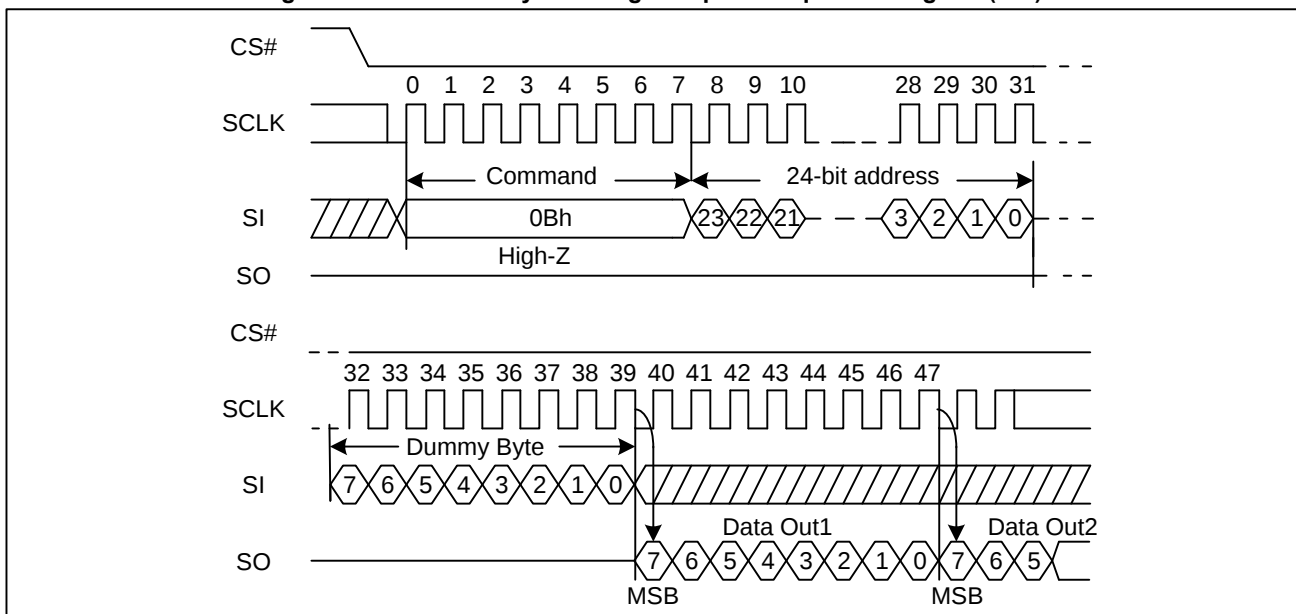
Figure 23. Read Data Bytes at Higher Speed Sequence Diagram (SPI)
