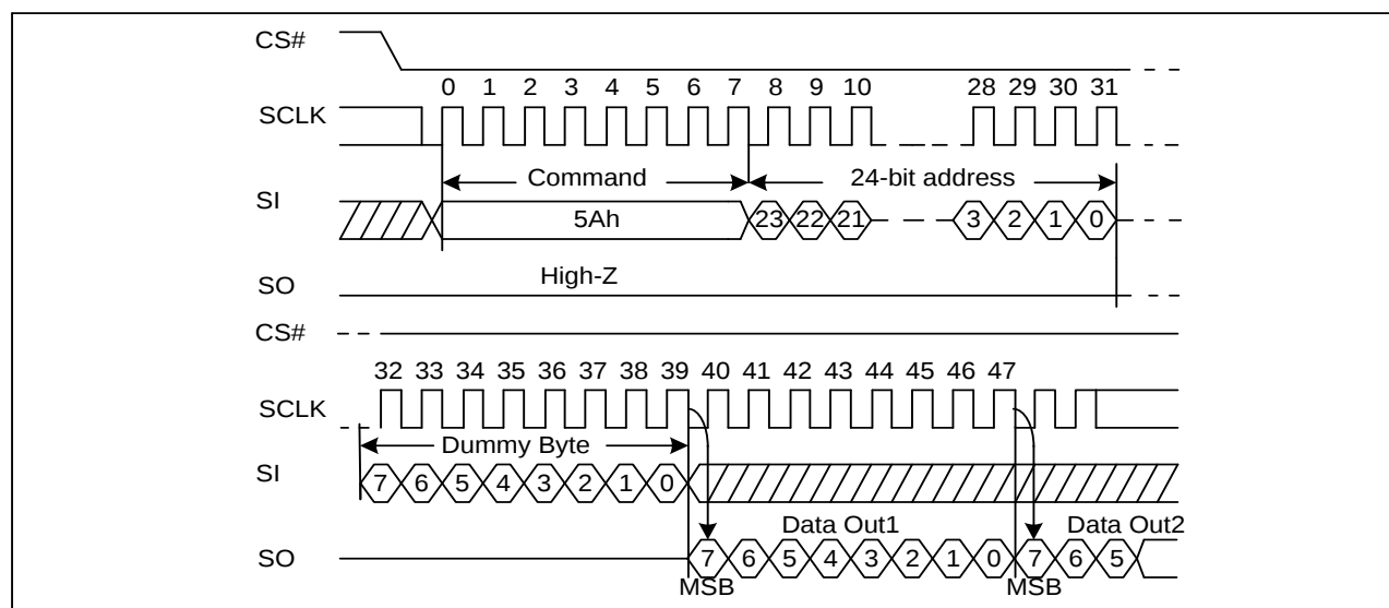
Figure 75. Read Serial Flash Discoverable Parameter command Sequence Diagram
