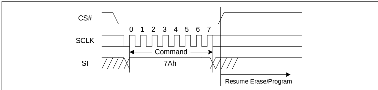
Figure 65. Program/Erase Resume Sequence Diagram (SPI)
