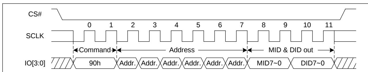
Figure 54. Read Manufacture ID/ Device ID Sequence Diagram (QPI)
