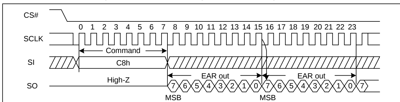
Figure 14. Read Extended Register Sequence Diagram (SPI)
