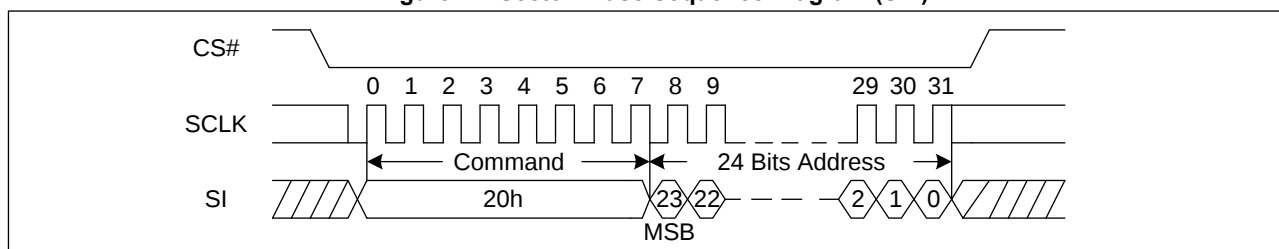
Figure 41. Sector Erase Sequence Diagram (SPI)
