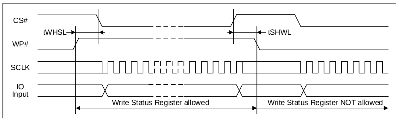
Figure 86. WP# Timing
