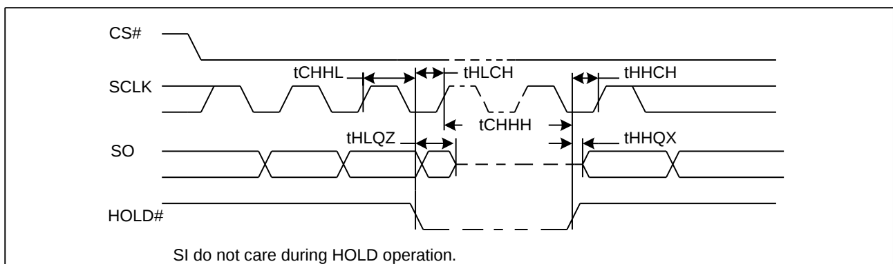
Figure 85. HOLD# Timing
