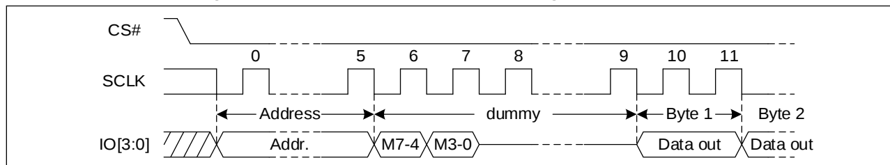
Figure 31. Quad I/O Fast Read Sequence Diagram ((M5-4) = (1, 0))
