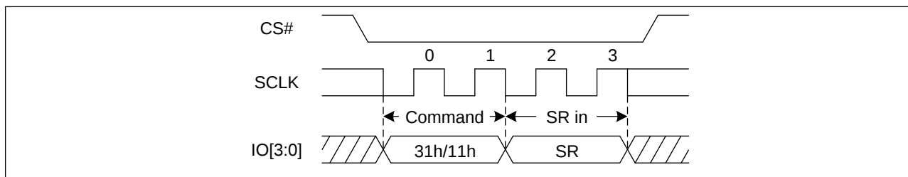
Figure 13. Write Status Register Sequence Diagram (QPI)
