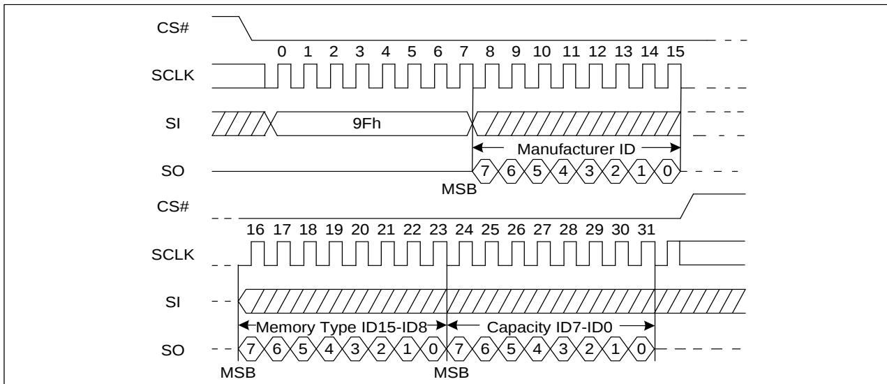
Figure 55. Read Identification ID Sequence Diagram (SPI)
