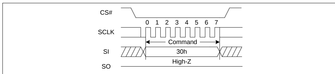
Figure 20. Clear Status Register Flags Sequence Diagram
