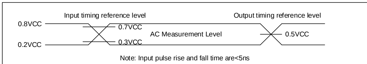
Figure 79. Absolute Maximum Ratings Diagram
