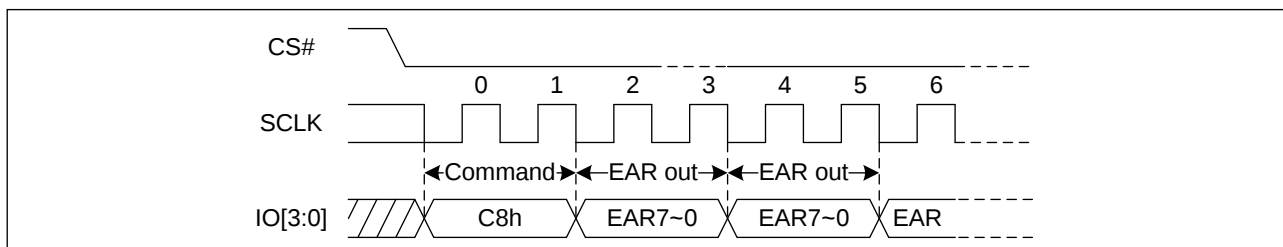
Figure 15. Read Extended Register Sequence Diagram (QPI)
