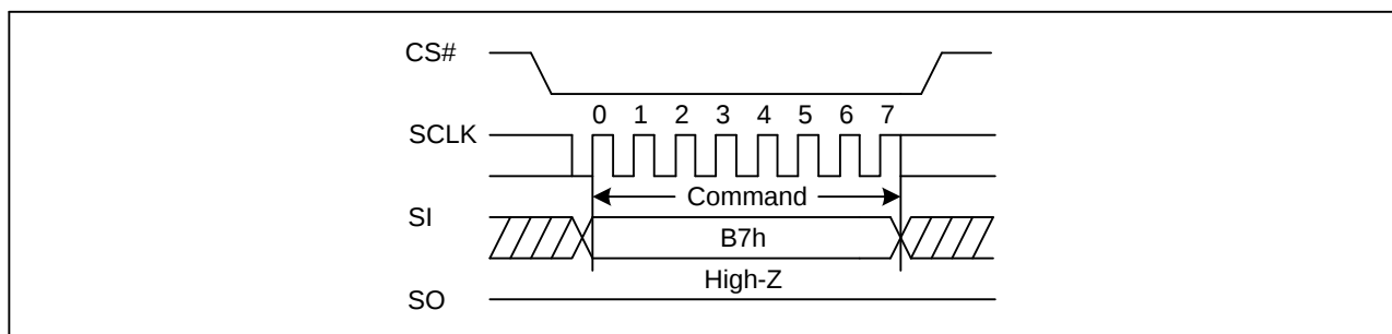
Figure 49 Enable 4-Byte Mode Sequence Diagram (SPI)
