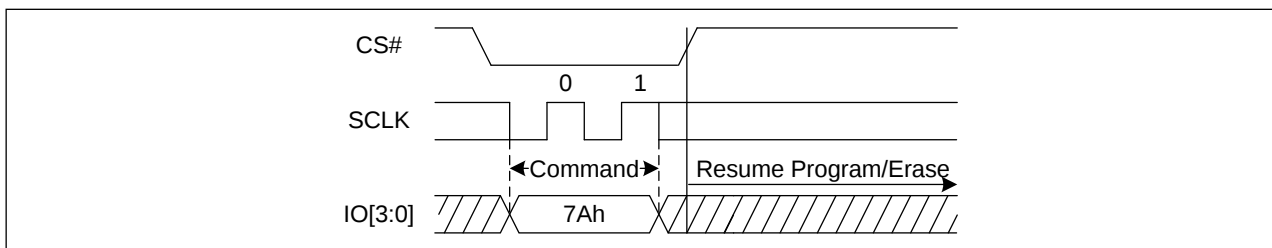
Figure 66. Program/Erase Resume Sequence Diagram (QPI)
