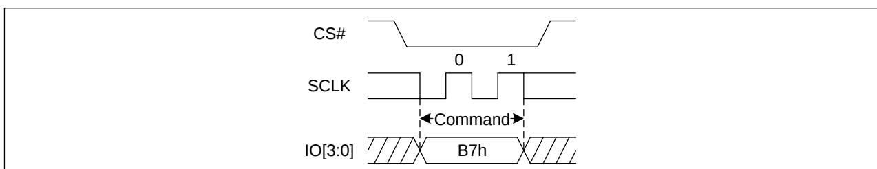
Figure 50 Enable 4-Byte Mode Sequence Diagram (QPI)
