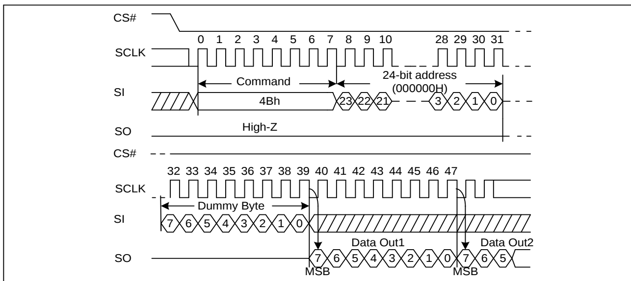
Figure 57. Read Unique ID Sequence Diagram
