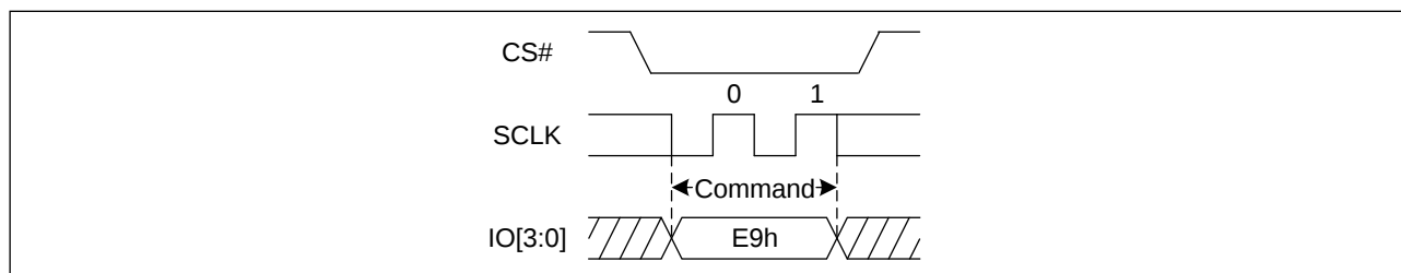
Figure 52 Disable 4-Byte Mode Sequence Diagram (QPI)
