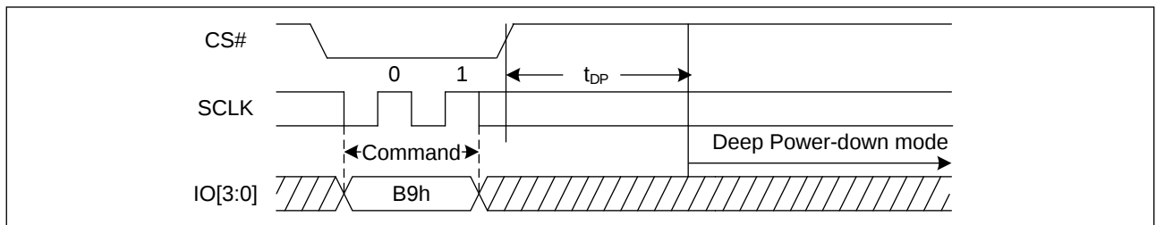
Figure 68. Deep Power-Down Sequence Diagram (QPI)
