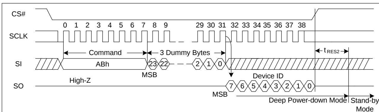
Figure 71. Release Power-Down/Read Device ID Sequence Diagram (SPI)
