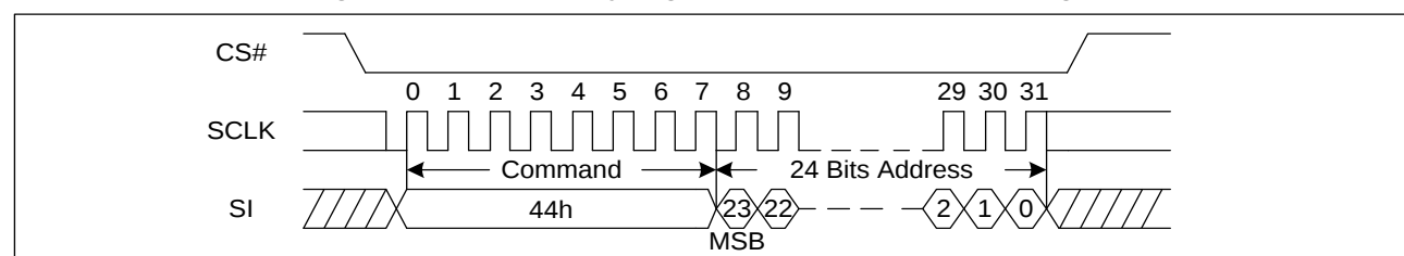
Figure 58. Erase Security Registers command Sequence Diagram
