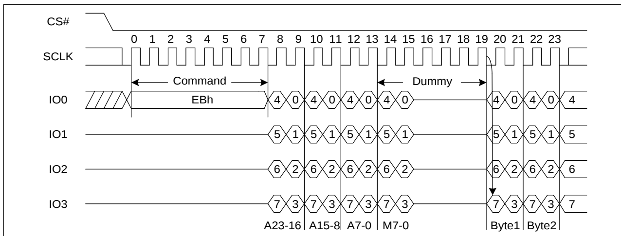
Figure 29. Quad I/O Fast Read Sequence Diagram ((M5-4) ≠ (1, 0), SPI)
