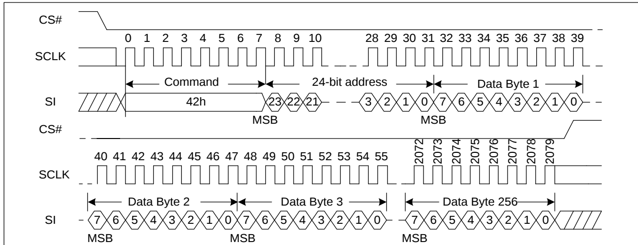
Figure 59. Program Security Registers command Sequence Diagram
