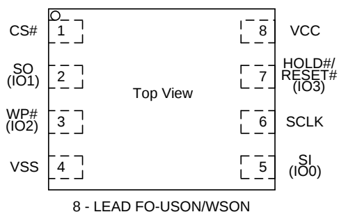
Figure 2 Connection Diagram for FO-USON8/WSN8 package
