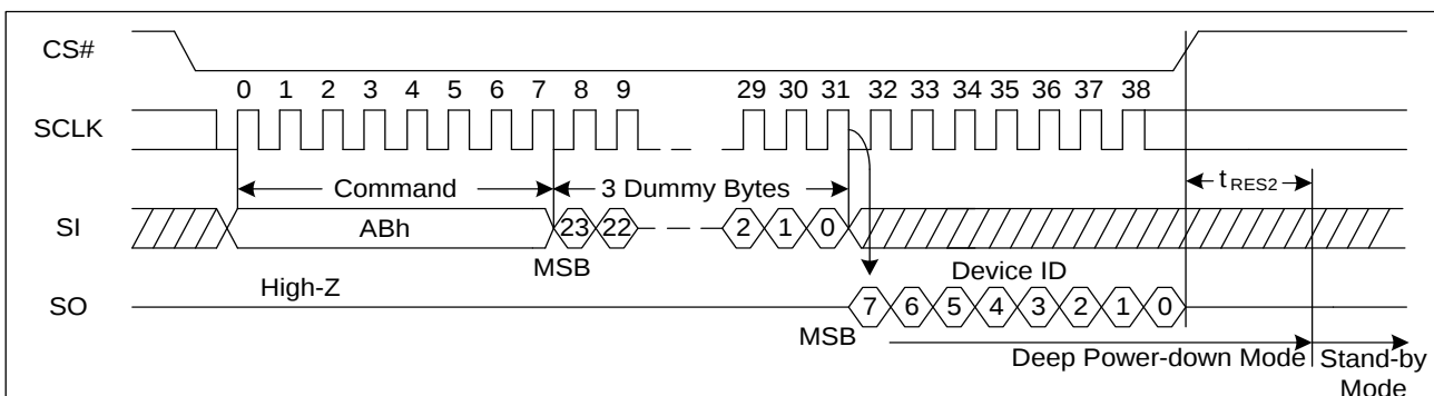
Figure 39. Release Power-Down/Read Device ID Sequence Diagram
