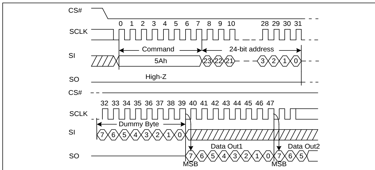
Figure 40. Read Serial Flash Discoverable Parameter command Sequence Diagram
