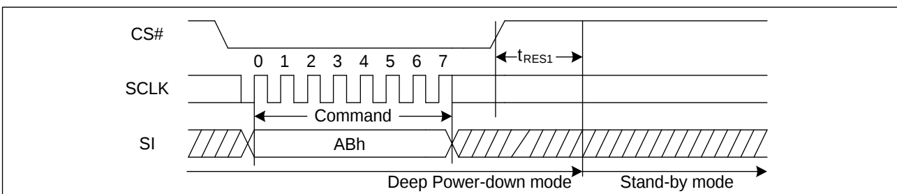
Figure 38. Release Power-Down Sequence Diagram
