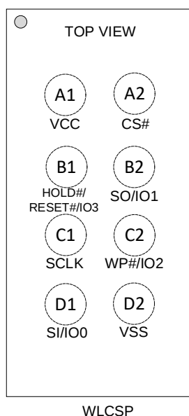
Figure 1 Connection Diagram for WLCSP package
