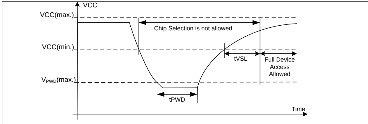
Figure 41. Power-Up/Down Timing Sequence Diagram
