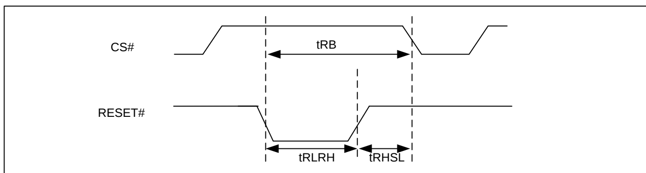
Figure 51. RESET# Timing
