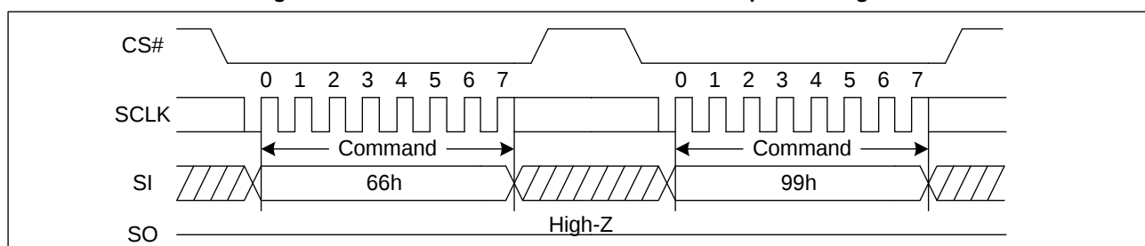
Figure 34. Enable Reset and Reset command Sequence Diagram
