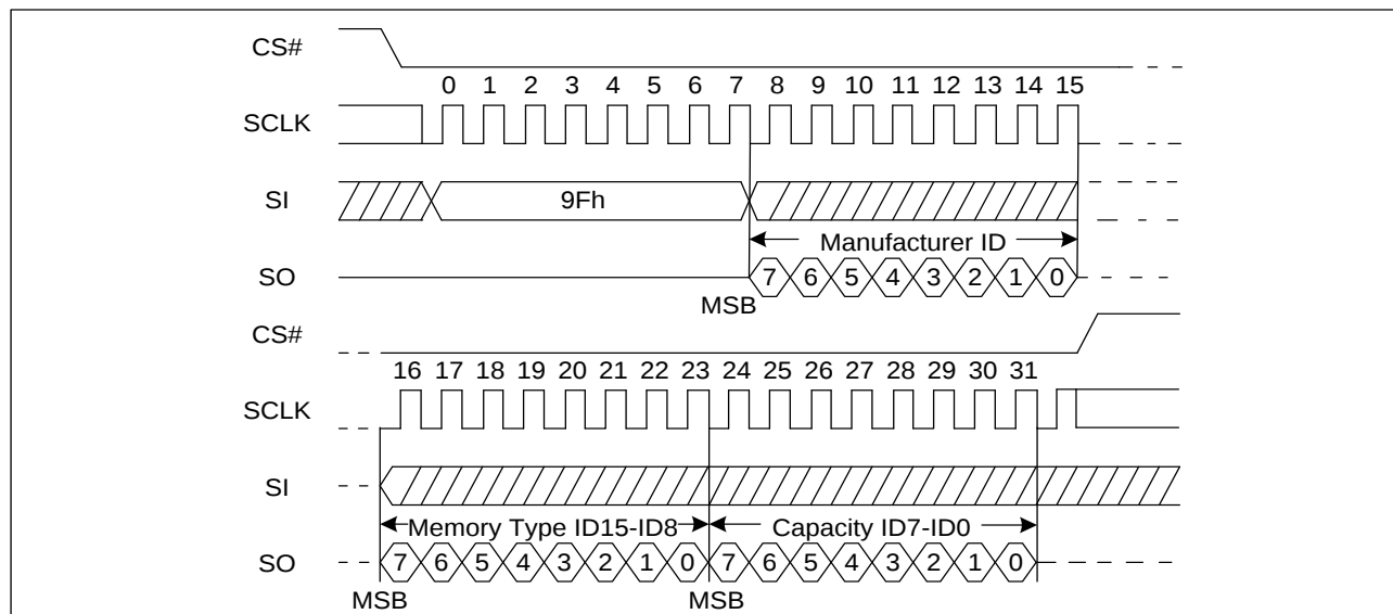
Figure 29. Read Identification ID Sequence Diagram
