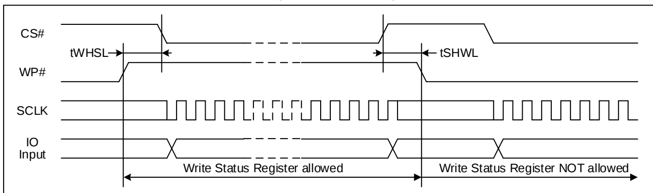
Figure 50. WP# Timing
