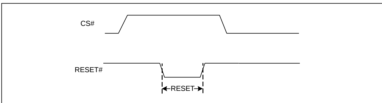
Figure 5 RESET Condition
