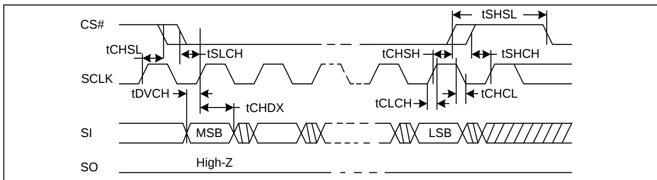
Figure 44. Input Timing
