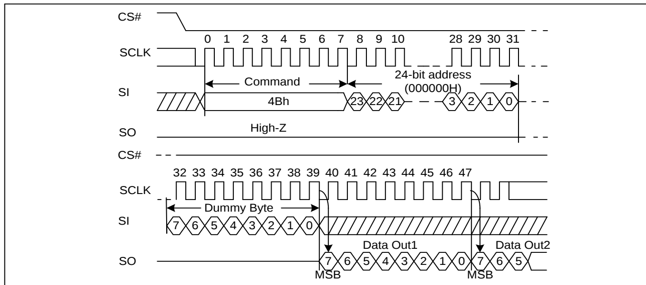
Figure 30. Read Unique ID Sequence Diagram
