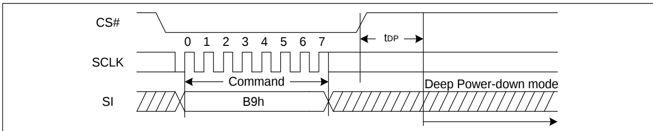
Figure 37. Deep Power-Down Sequence Diagram
