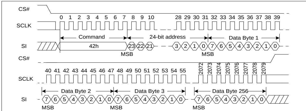
Figure 32. Program Security Registers command Sequence Diagram
