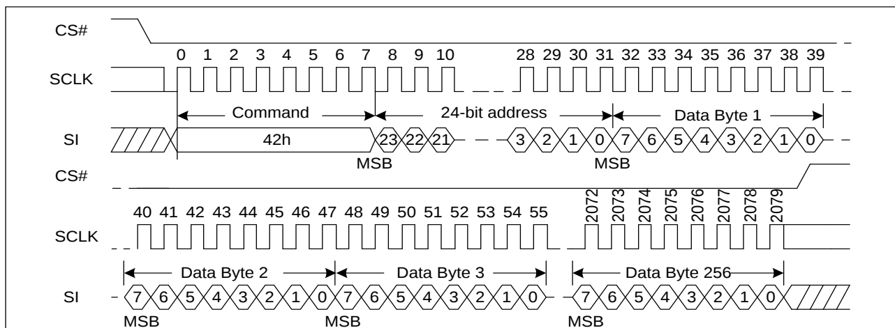
Figure 29. Program Security Registers command Sequence Diagram
