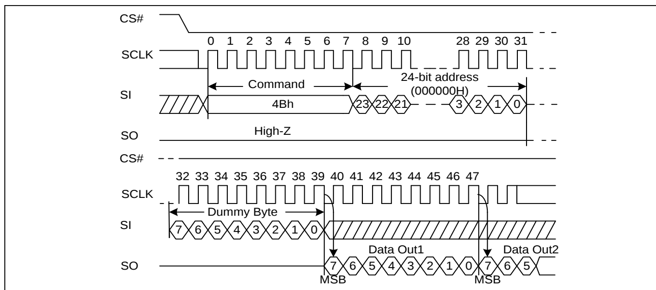
Figure 27. Read Unique ID Sequence Diagram
