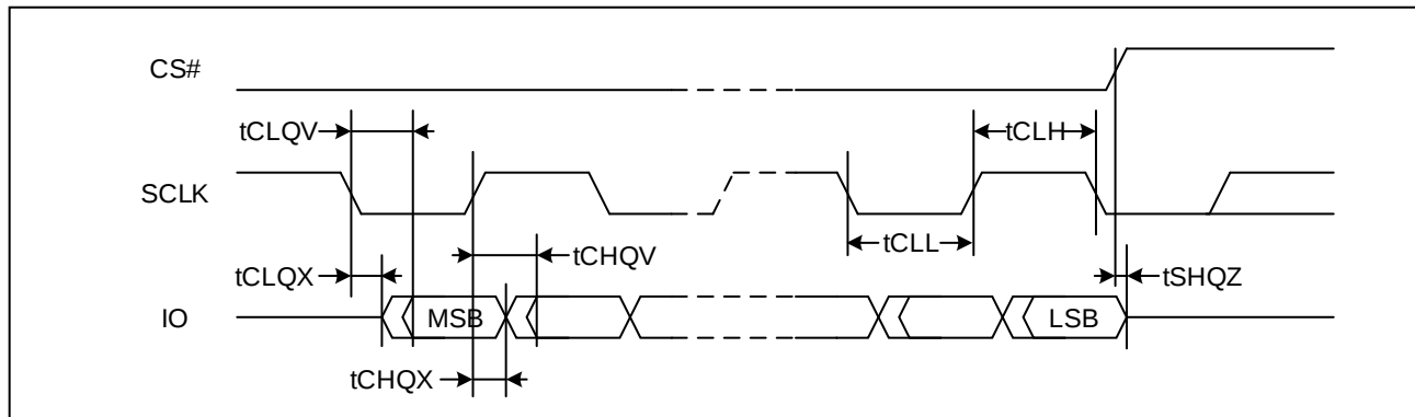
Figure 44. Serial Output Timing (DTR)
