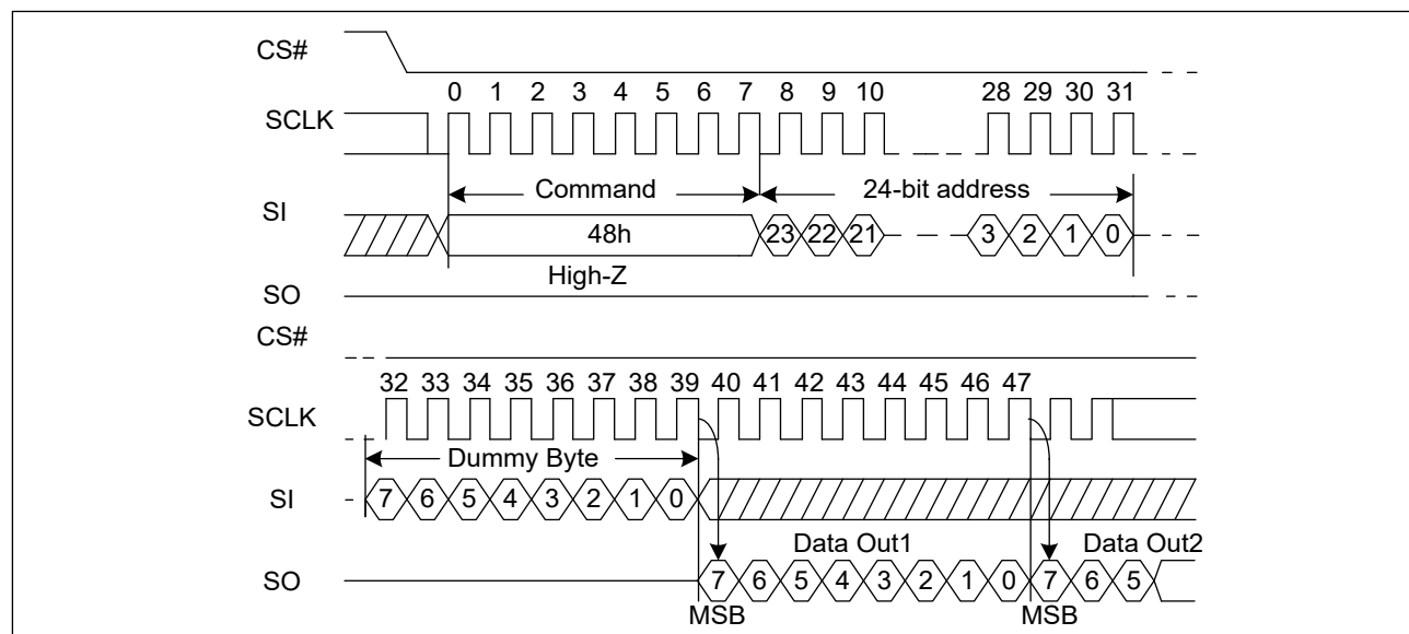
Figure 59. Read Security Registers command Sequence Diagram
