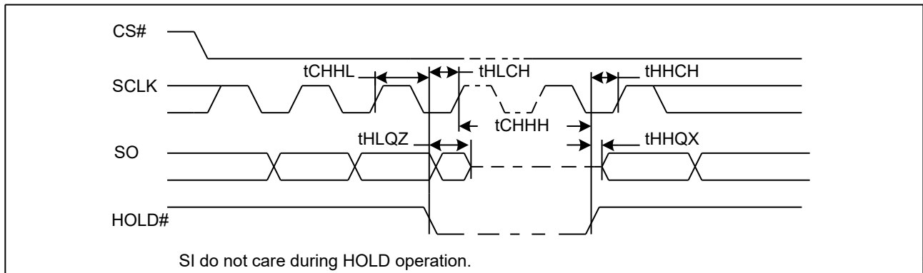
Figure 84. HOLD# Timing
