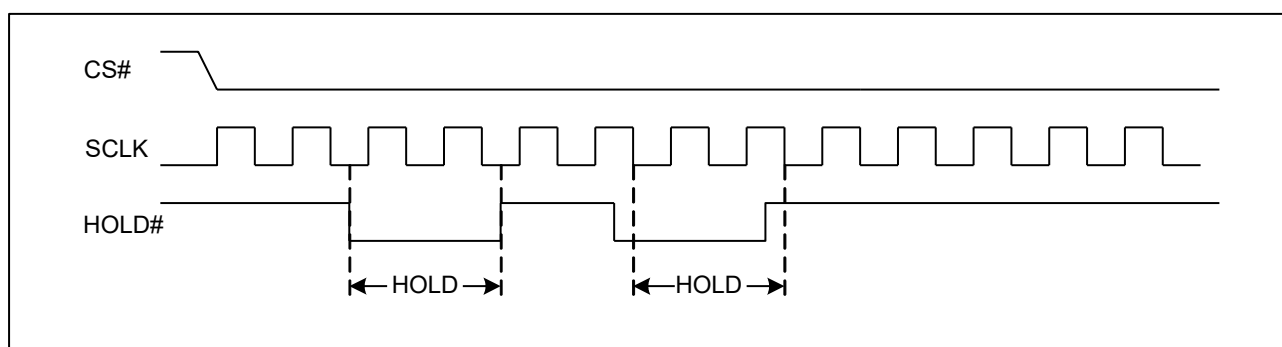
Figure 5 HOLD Condition
