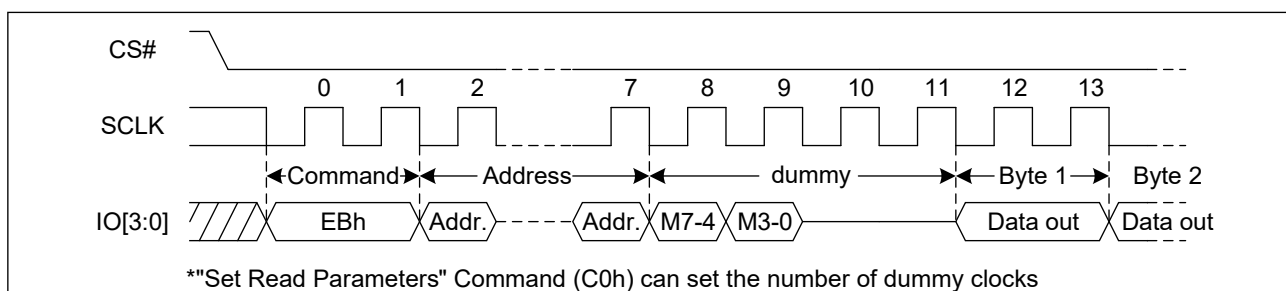
Figure 32. Quad I/O Fast Read Sequence Diagram ((M5-4) ≠ (1, 0), QPI)
