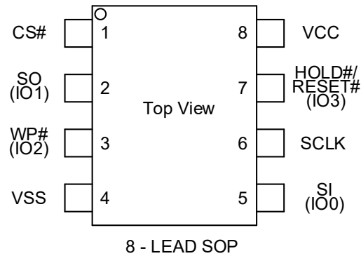
Figure 4 Connection Diagram for SOP8 package
