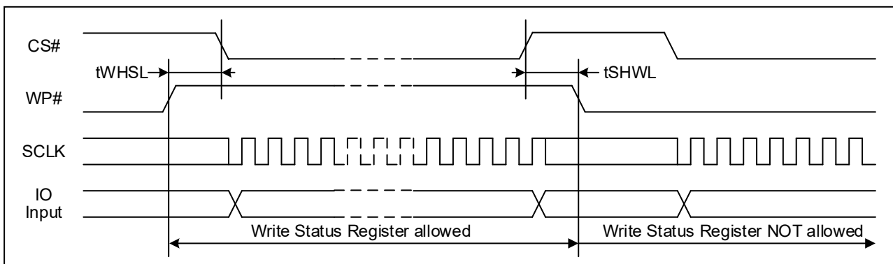
Figure 83. WP# Timing
