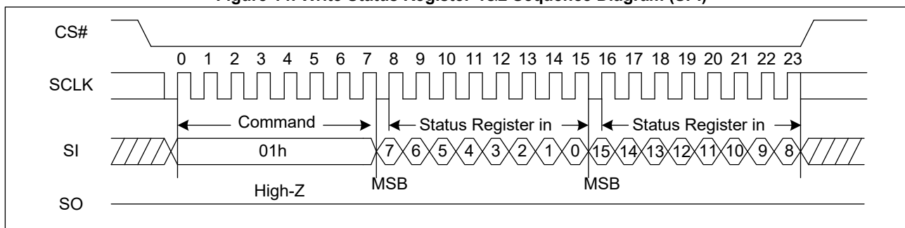
Figure 14. Write Status Register-1&2 Sequence Diagram (SPI)
