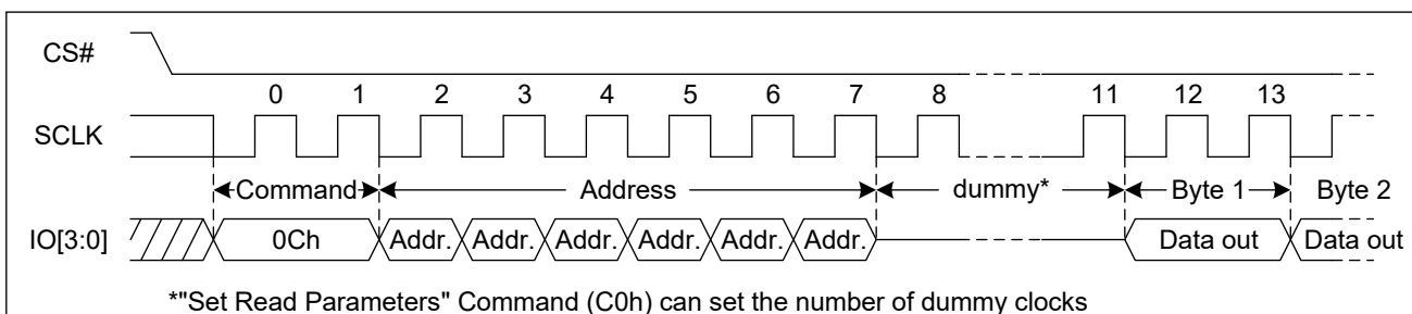
Figure 37. Burst Read with Wrap Sequence Diagram
