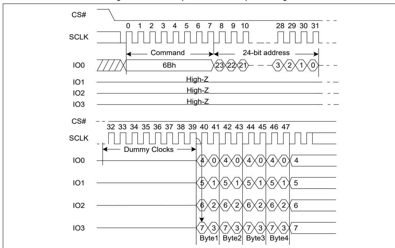
Figure 30. Quad Output Fast Read Sequence Diagram
