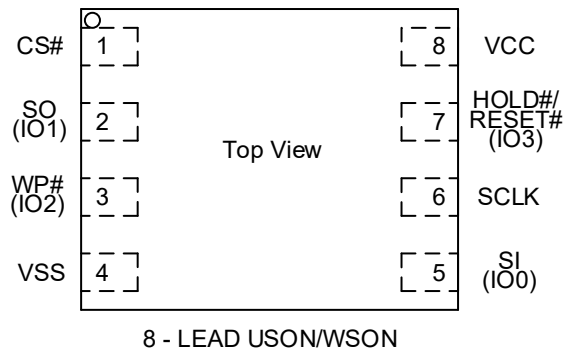
Figure 3 Connection Diagram for USON8/WSO8 package
