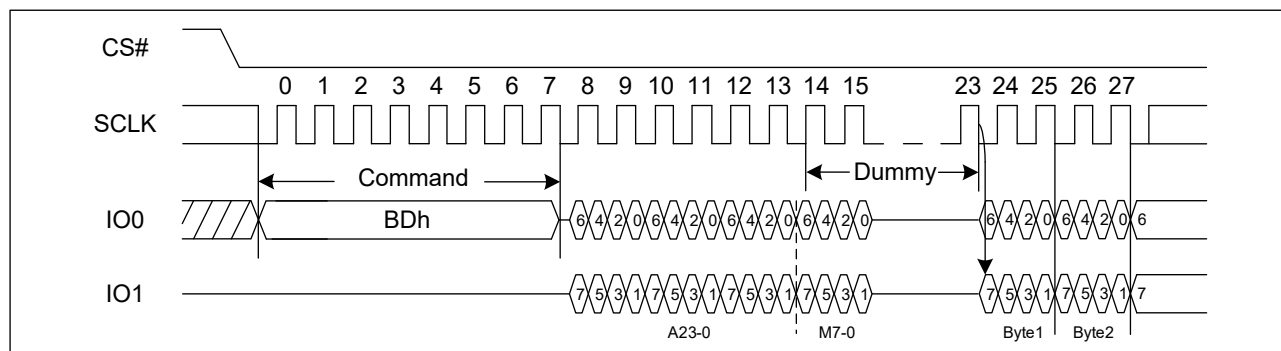
Figure 28. DTR Dual I/O Fast Read Sequence Diagram (M5-4 ≠ (1, 0))
