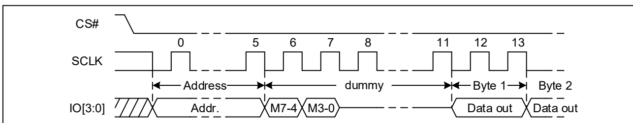
Figure 33. Quad I/O Fast Read Sequence Diagram ((M5-4) = (1, 0))
