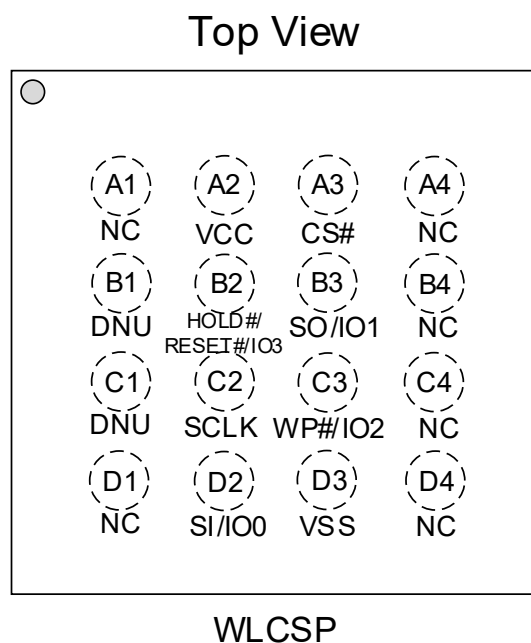
Figure 2 Connection Diagram for WLCSP 4-4 ball array package
