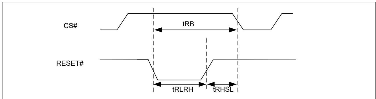
Figure 85. RESET# Timing
