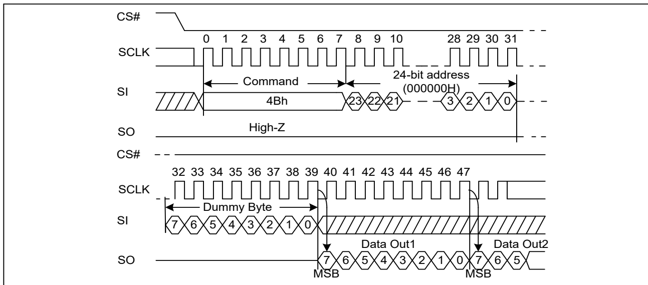
Figure 56. Read Unique ID Sequence Diagram
