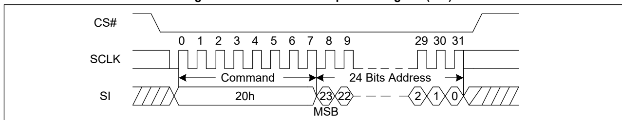
Figure 44. Sector Erase Sequence Diagram (SPI)
