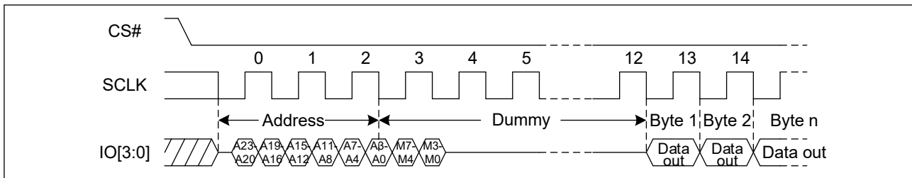
Figure 32. DTR Quad I/O Fast Read Sequence Diagram (M5-4 = (1, 0))
