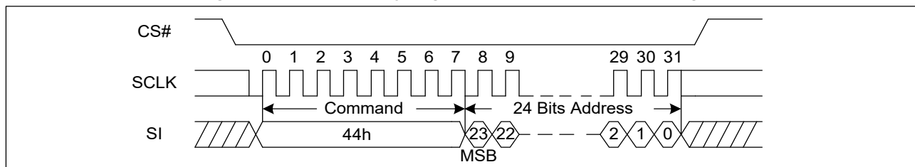
Figure 53. Erase Security Registers command Sequence Diagram
