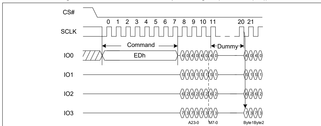
Figure 30. DTR Quad I/O Fast Read Sequence Diagram (SPI, M5-4≠ (1, 0))
