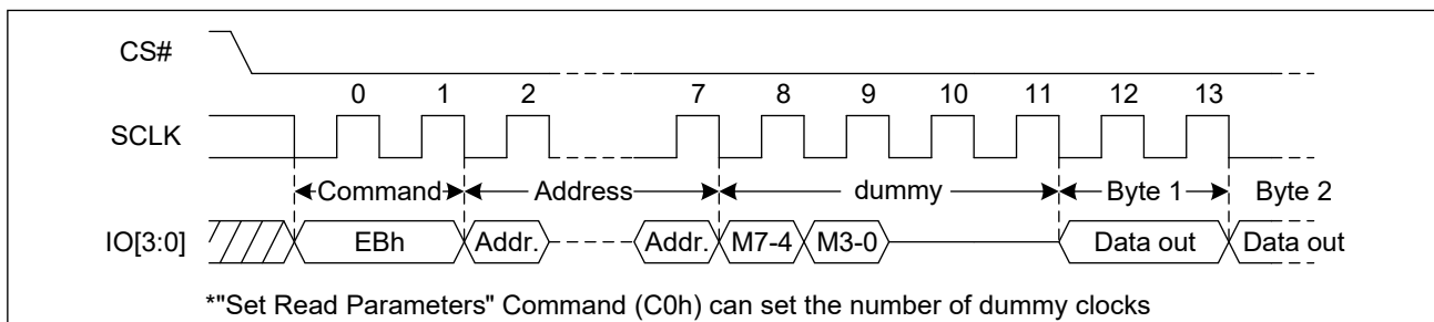
Figure 28. Quad I/O Fast Read Sequence Diagram ((M5-4) ≠ (1, 0), QPI)
