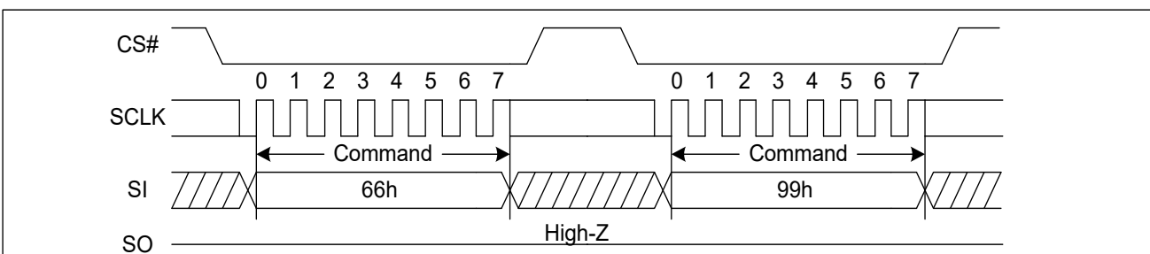
Figure 56. Enable Reset and Reset command Sequence Diagram (SPI)
