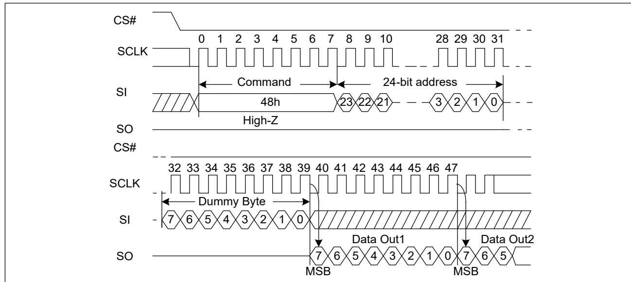
Figure 55. Read Security Registers command Sequence Diagram
