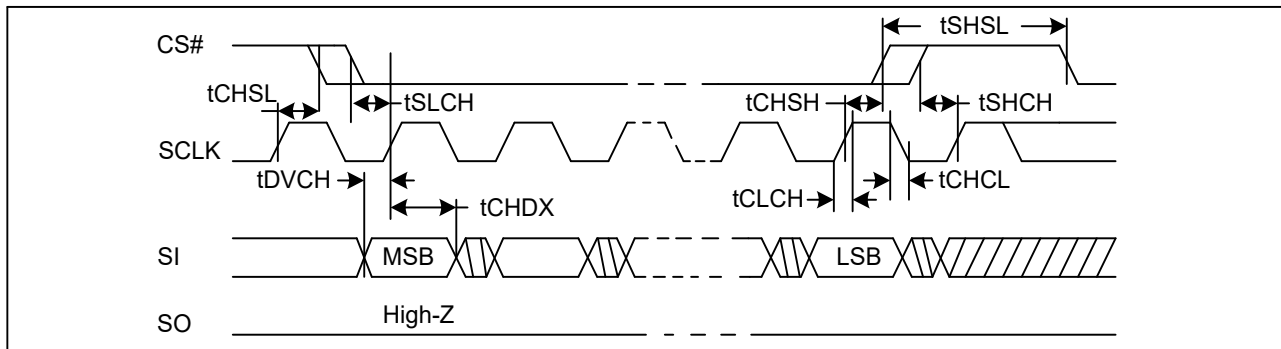
Figure 74. Serial Input Timing (STR)
