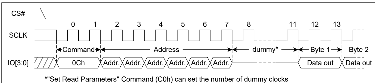
Figure 33. Burst Read with Wrap Sequence Diagram
