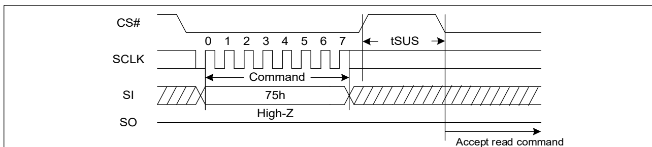
Figure 58. Program/Erase Suspend Sequence Diagram (SPI)
