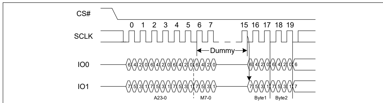
Figure 25. DTR Dual I/O Fast Read Sequence Diagram (M5-4 = (1, 0))
