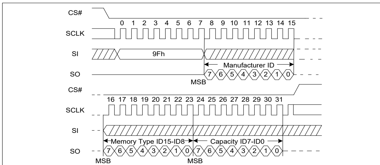
Figure 50. Read Identification ID Sequence Diagram (SPI)
