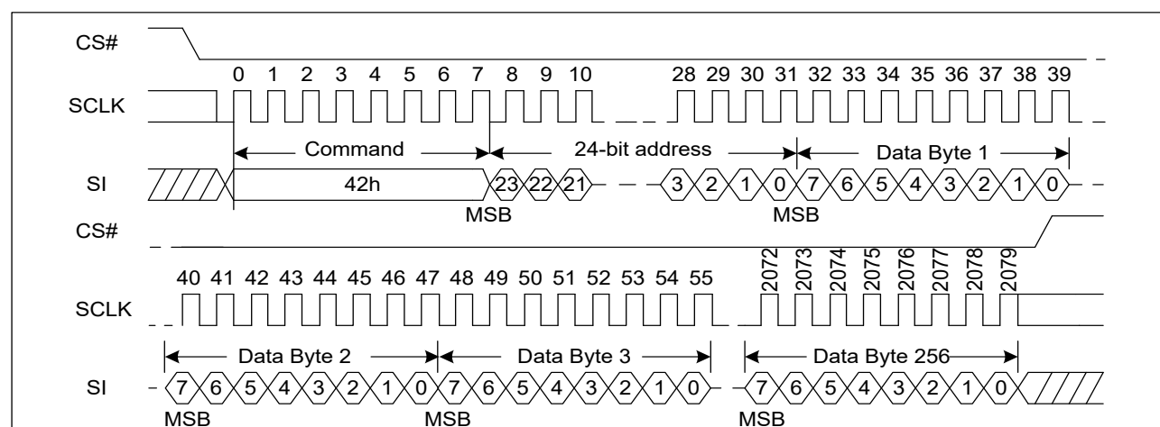
Figure 54. Program Security Registers command Sequence Diagram
