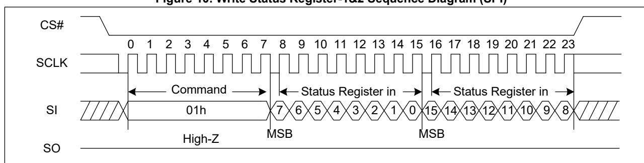
Figure 10. Write Status Register-1&2 Sequence Diagram (SPI)
