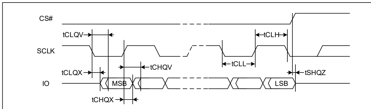
Figure 77. Serial Output Timing (DTR)
