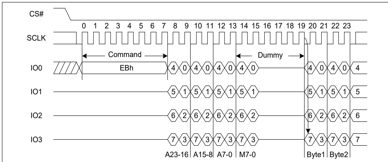
Figure 27. Quad I/O Fast Read Sequence Diagram ((M5-4) ≠ (1, 0), SPI)
