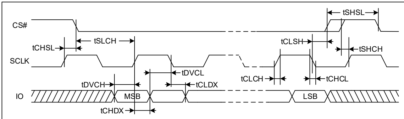
Figure 76. Serial Input Timing (DTR)
