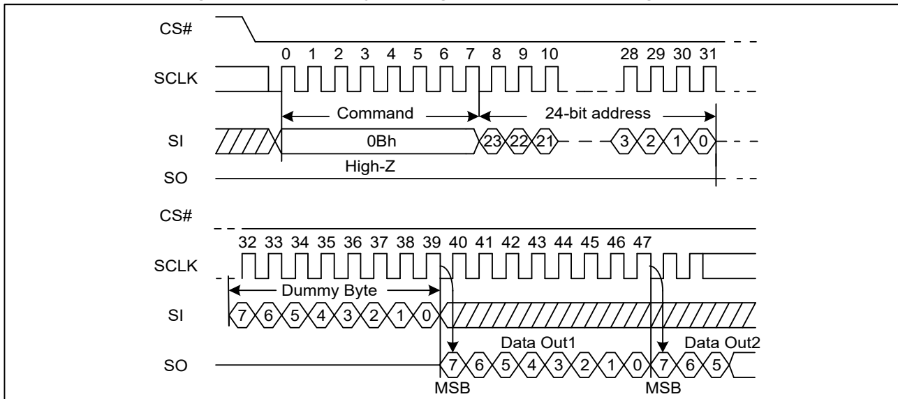
Figure 19. Read Data Bytes at Higher Speed Sequence Diagram (SPI)
