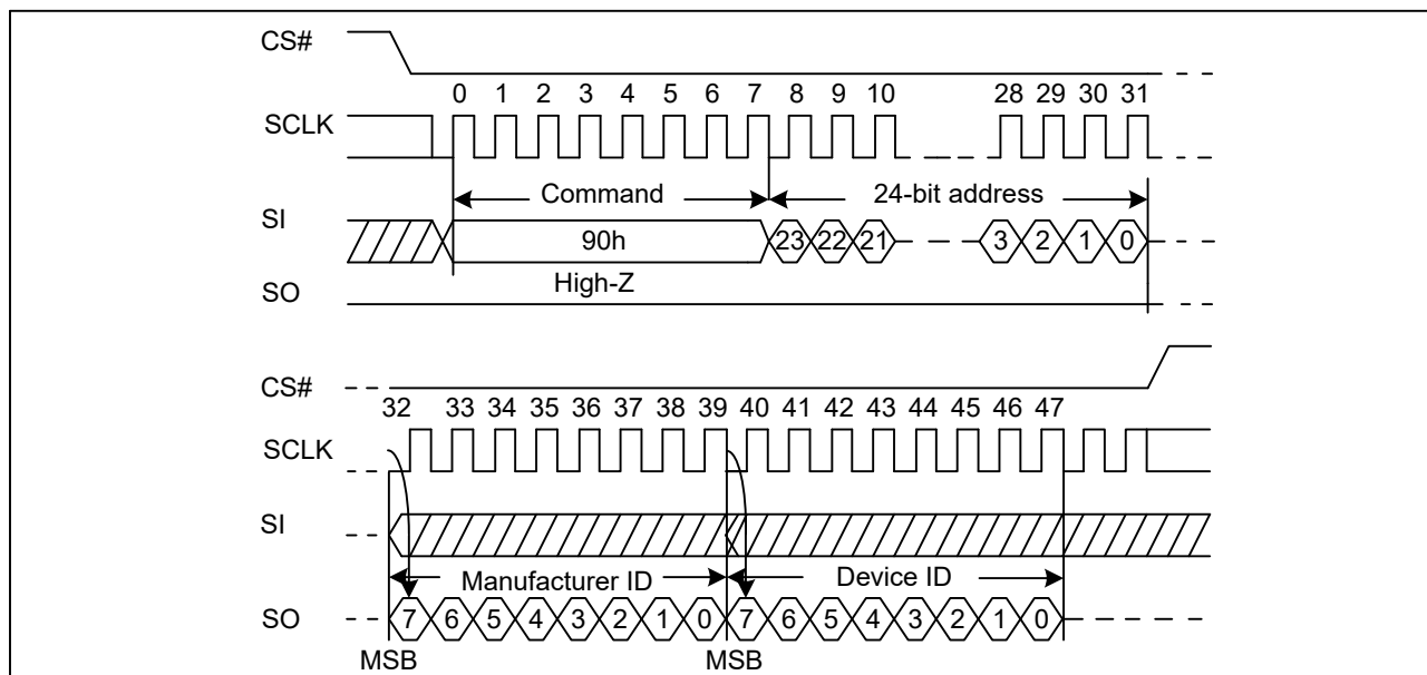
Figure 48. Read Manufacture ID/ Device ID Sequence Diagram (SPI)
