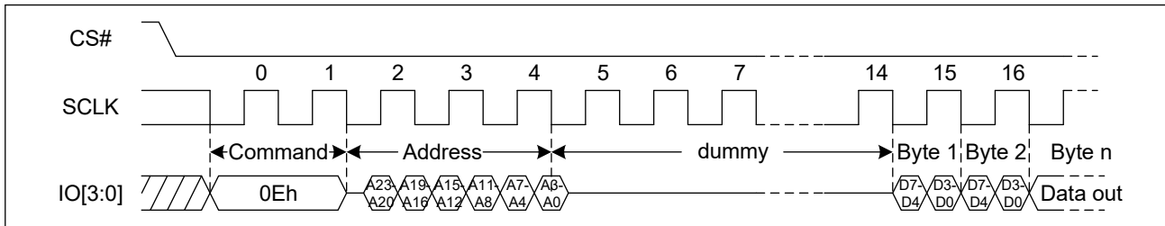
Figure 34. DTR Burst Read with Wrap Sequence Diagram
