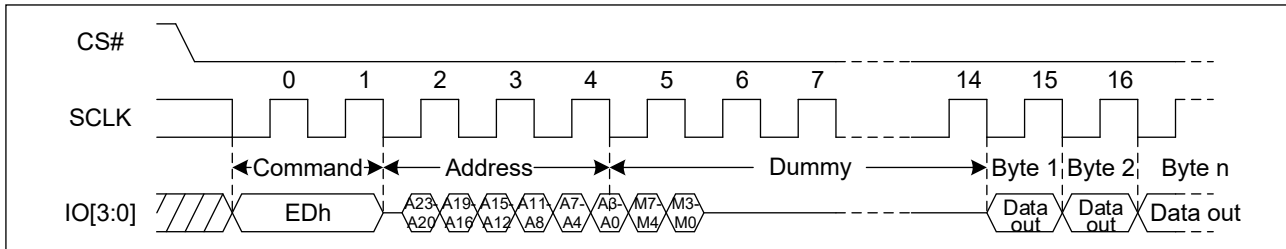
Figure 31. DTR Quad I/O Fast Read Sequence Diagram (QPI, M5-4# (1, 0))
