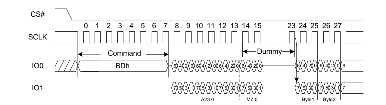
Figure 24. DTR Dual I/O Fast Read Sequence Diagram (M5-4 ≠ (1, 0))
