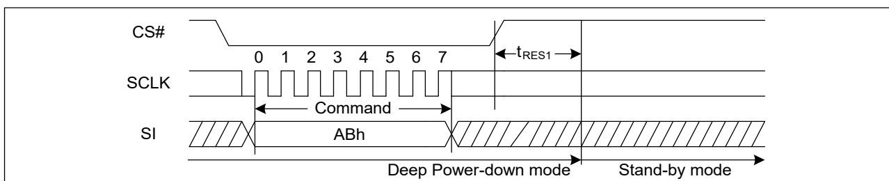
Figure 64. Release Power-Down Sequence Diagram (SPI)
