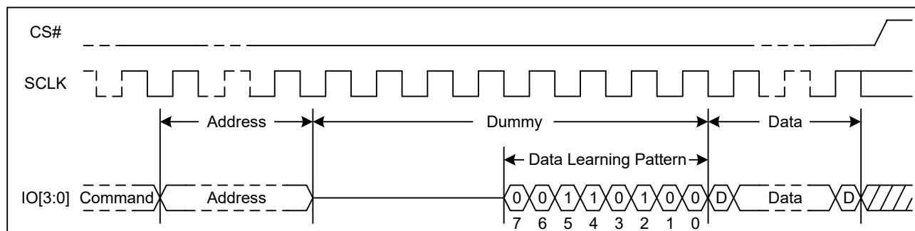
Figure 3. Data Learning Pattern Sequence Diagram (DTR, Dummy Clock ≥ 8)
