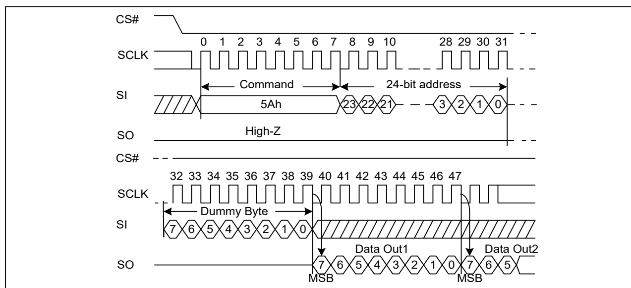
Figure 70. Read Serial Flash Discoverable Parameter command Sequence Diagram
