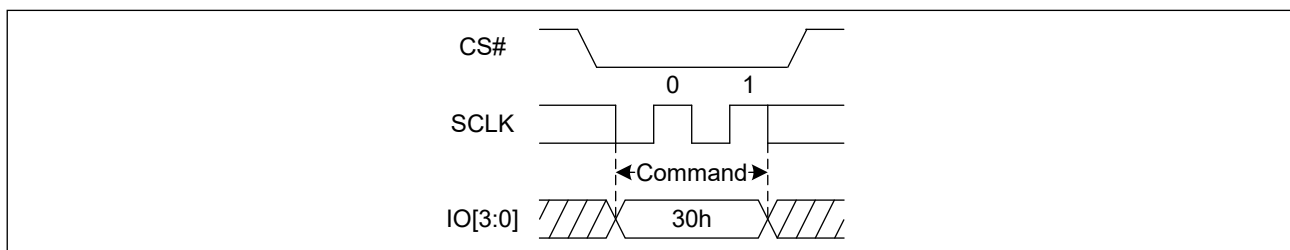
Figure 17. Clear Status Register Flags Sequence Diagram (QPI)
