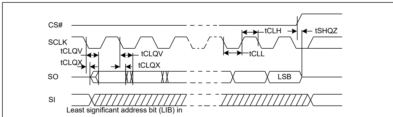
Figure 75. Serial Output Timing (STR)
