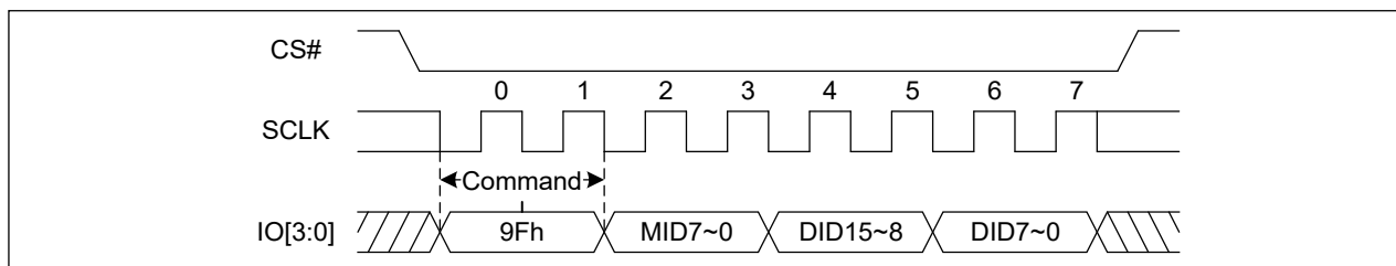
Figure 51. Read Identification ID Sequence Diagram (QPI)
