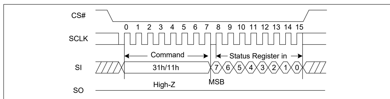
Figure 12. Write Status Register Sequence Diagram (SPI)
