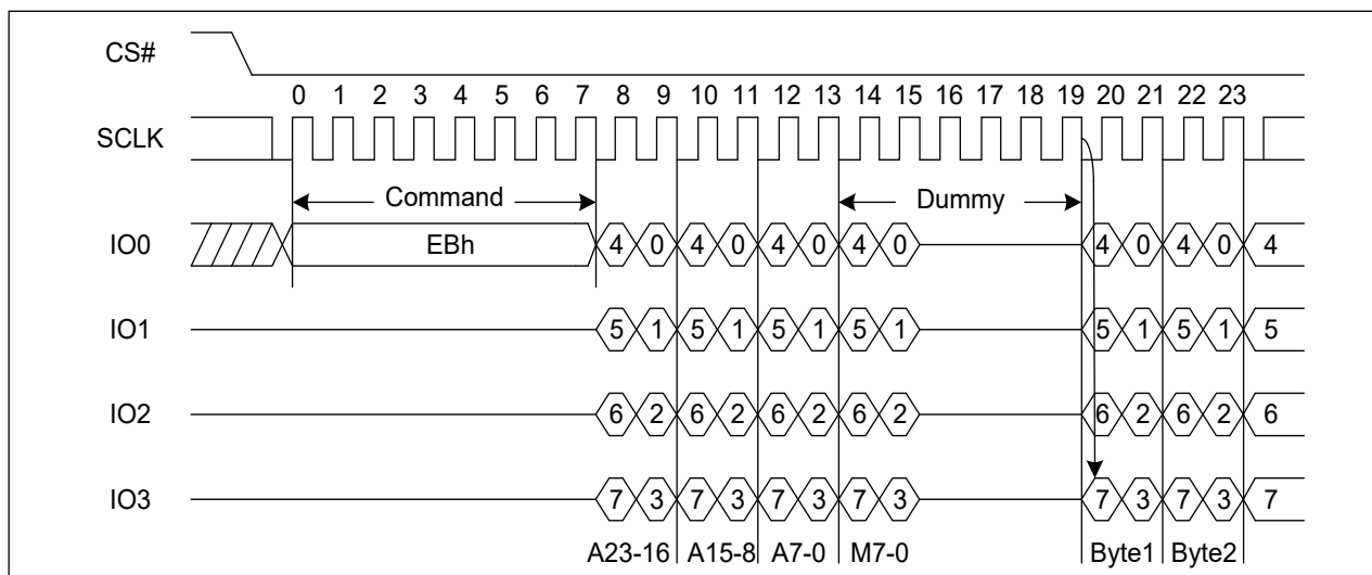
Figure 26. Quad I/O Fast Read Sequence Diagram ((M5-4) ≠ (1, 0), SPI)
