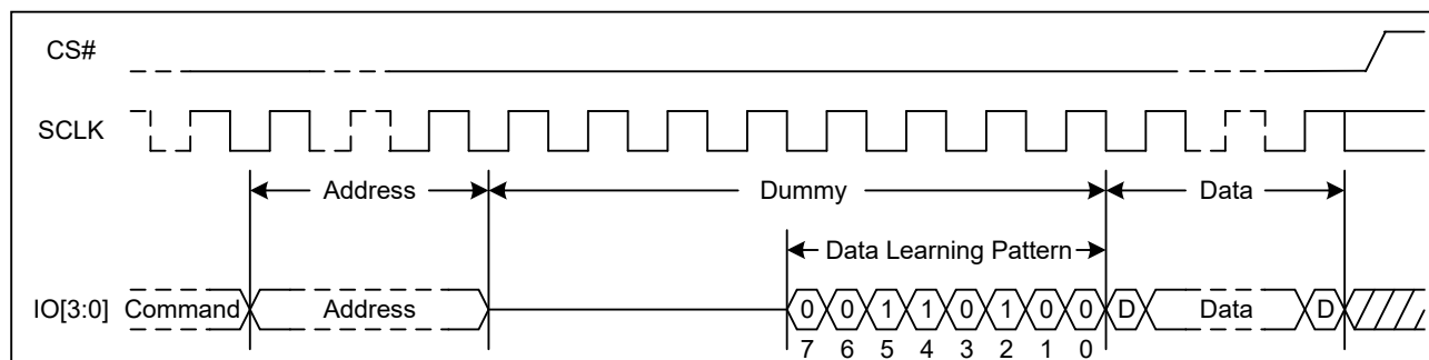
Figure 4. Data Learning Pattern Sequence Diagram (DTR, Dummy Clock ≥ 8)
