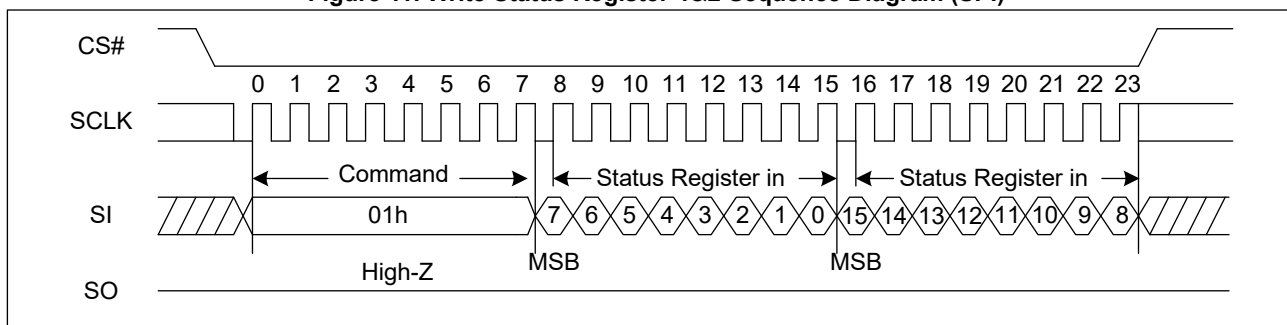
Figure 11. Write Status Register-1&2 Sequence Diagram (SPI)
