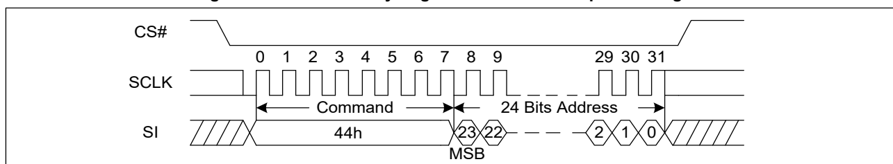
Figure 54. Erase Security Registers command Sequence Diagram
