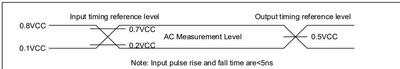
Figure 74. Absolute Maximum Ratings Diagram
