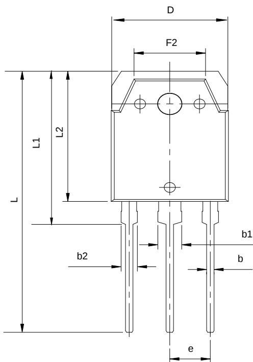
TO-247S-3L
