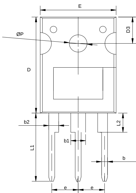
TO-247S-3L
