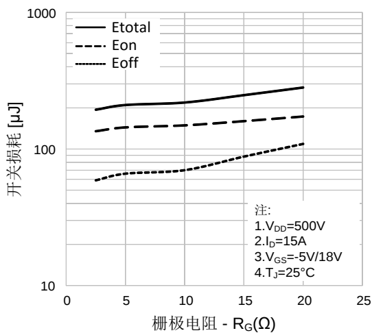
图21. 开关损耗 vs. 栅极电阻
