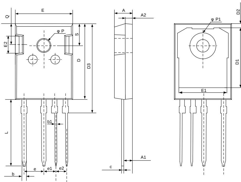
TO-247N-4L
