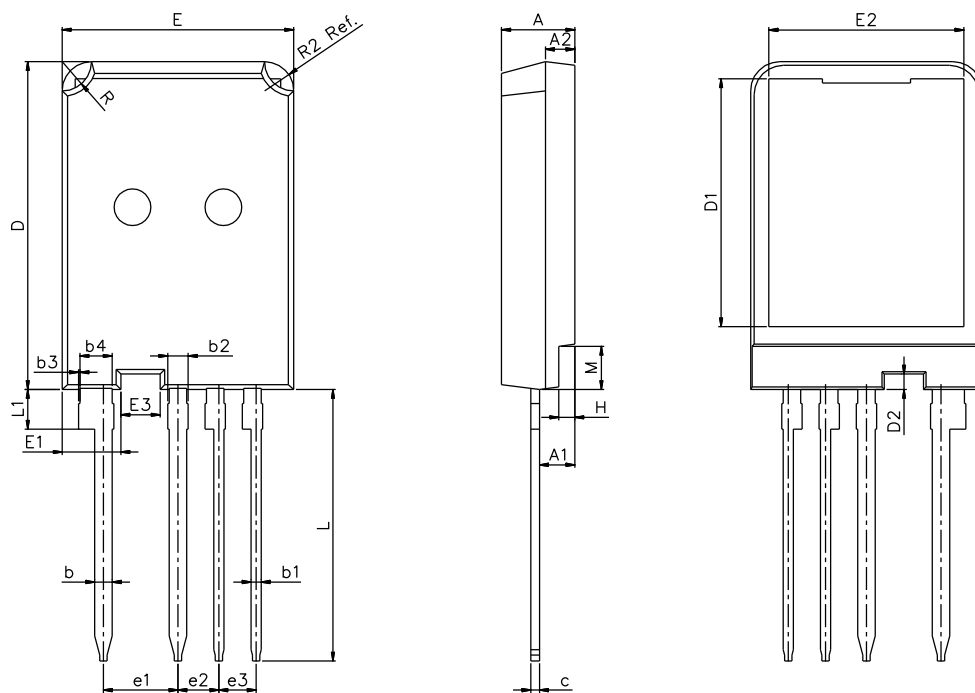
TO-247PJ-4L
