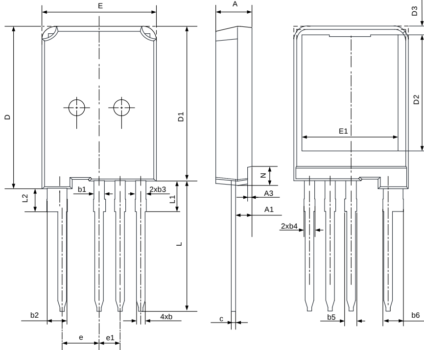
TO-247PJ-4L
