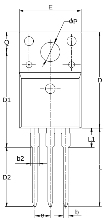
TO-220FJD-3L
