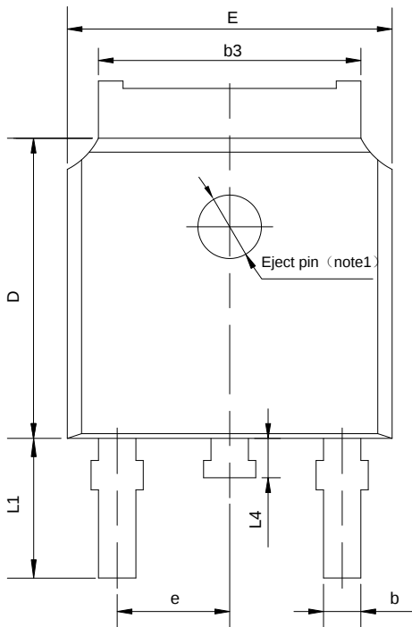
TO-252-2L
