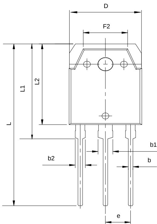
TO-3P
