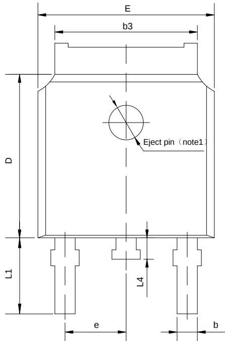
TO-252-2L
