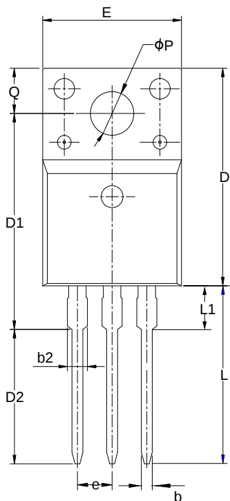
TO-220F-3L
