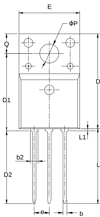
TO-220FJH-3L
