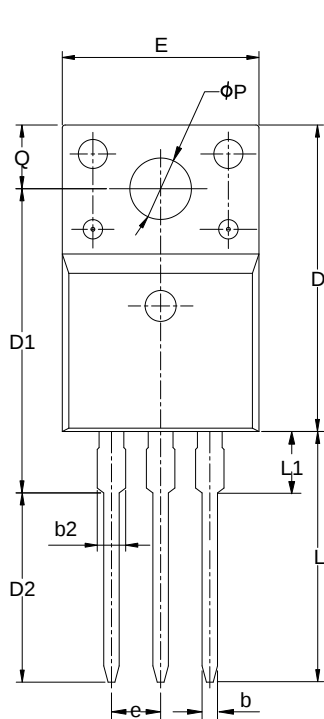
TO-220FJD-3L
