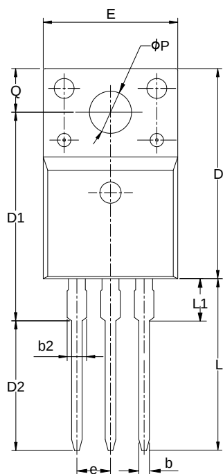
TO-220FJD-3L
