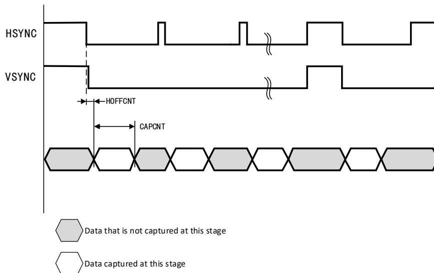
Figure 25-6 Crop window data capture waveform
