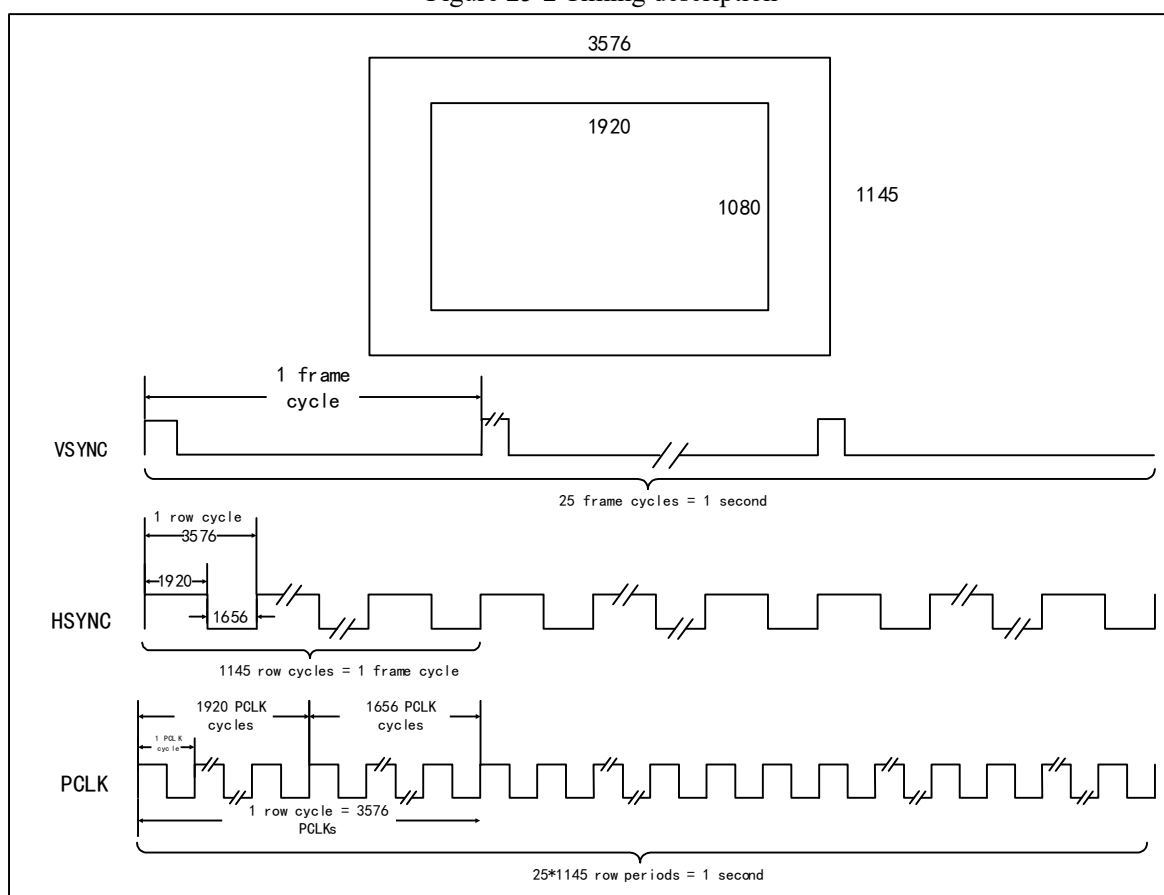
Figure 25-2 Timing description
