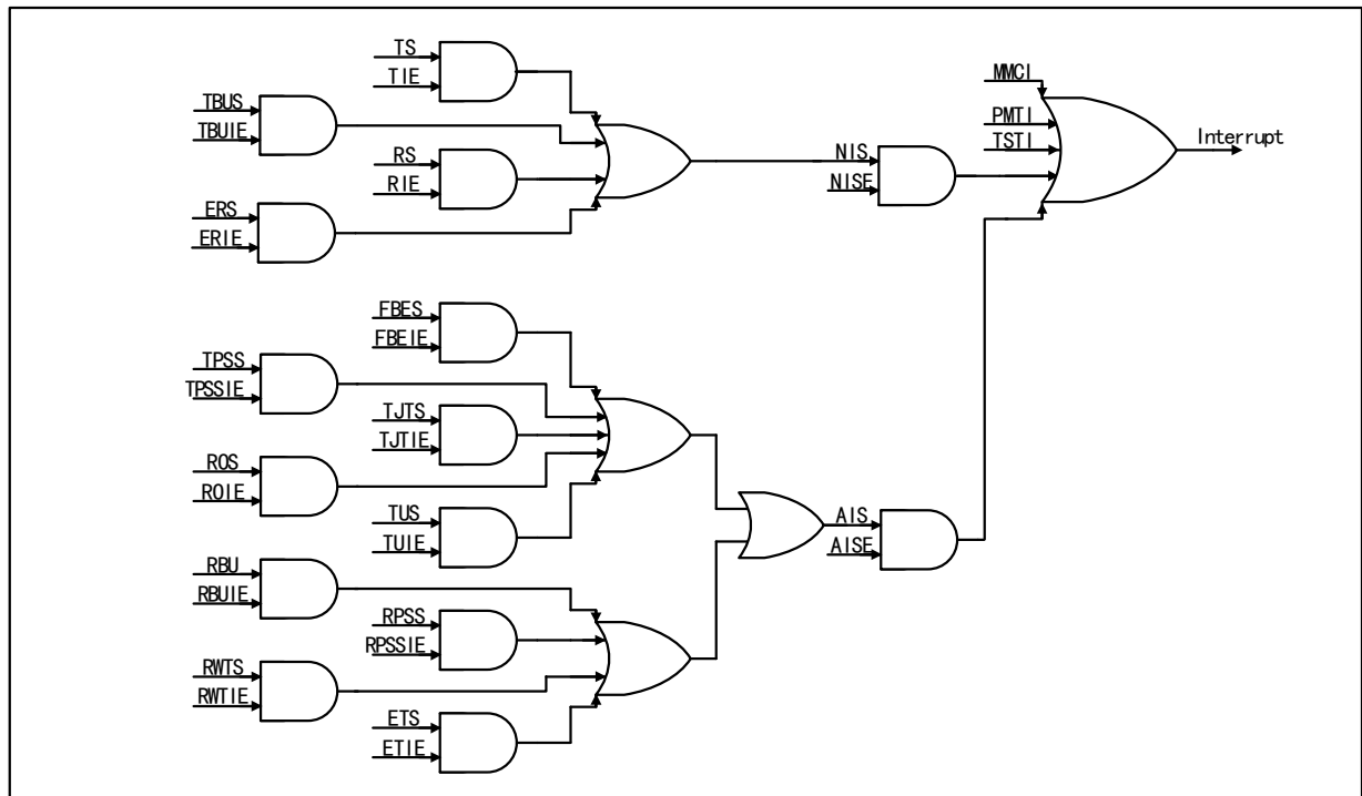
Figure 27-13 Interrupt schematic
