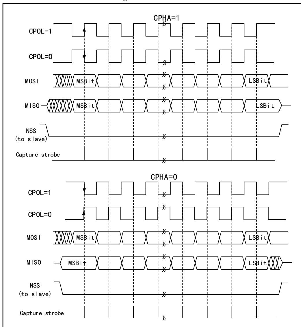
Figure 20-2 SPI model
