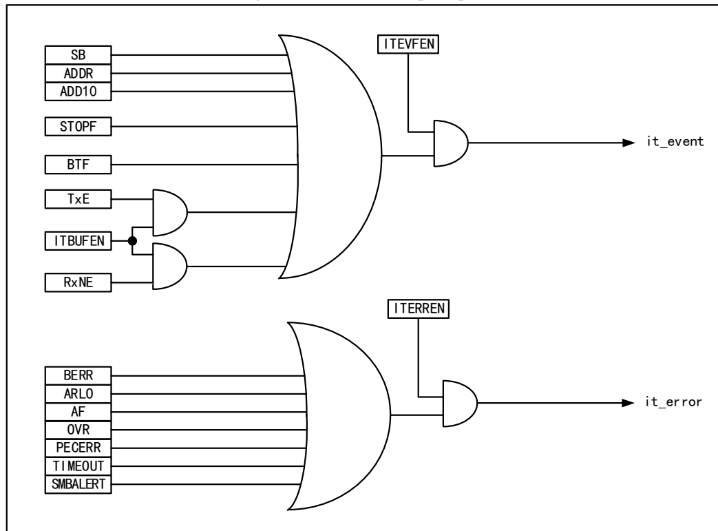
Figure 19-4 I2C interrupt request
