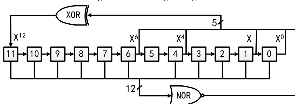
Figure 17-5 LFSR register algorithm
