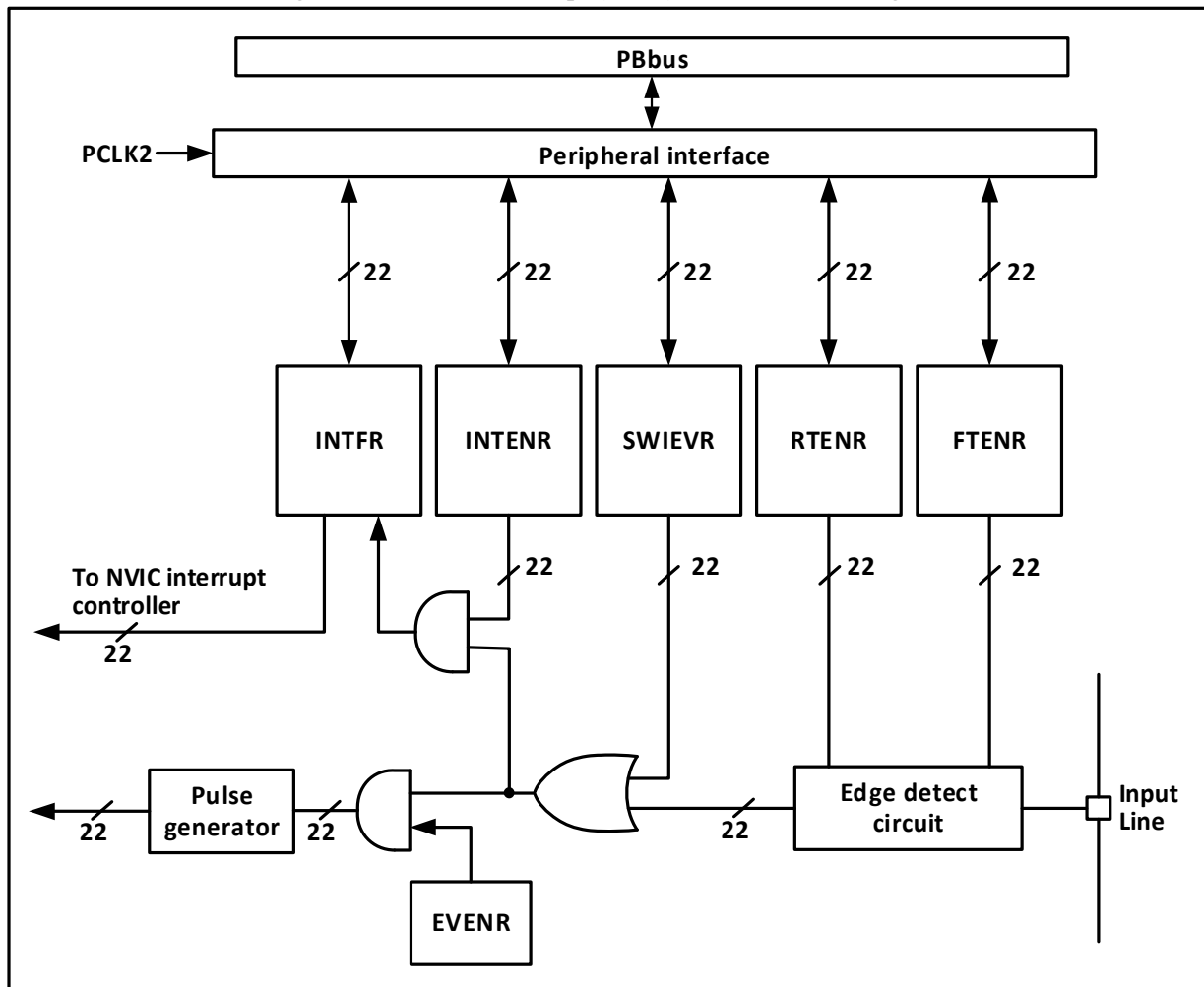
Figure 9-1 External interrupt (EXTI) interface block diagram
