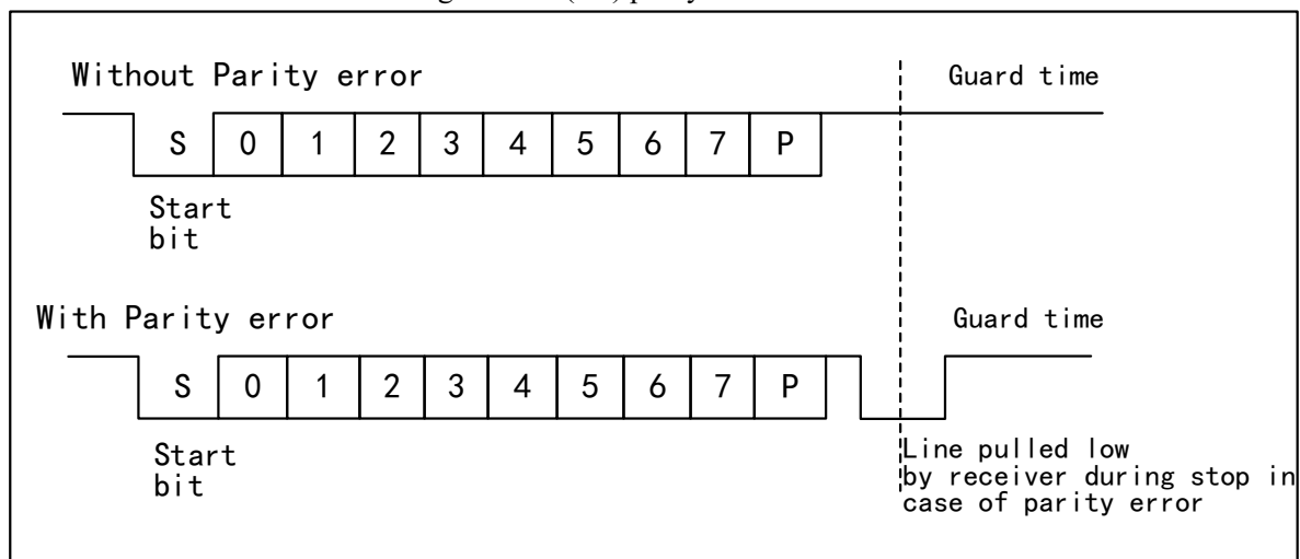
Figure 18-4 (No) parity check error
