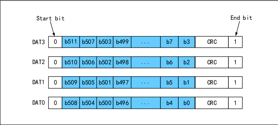
Figure 28-12 SD card 4 bus data transfer in a 512-bit word format
