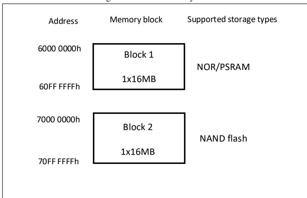
Figure 26-2 FSMC memory block
