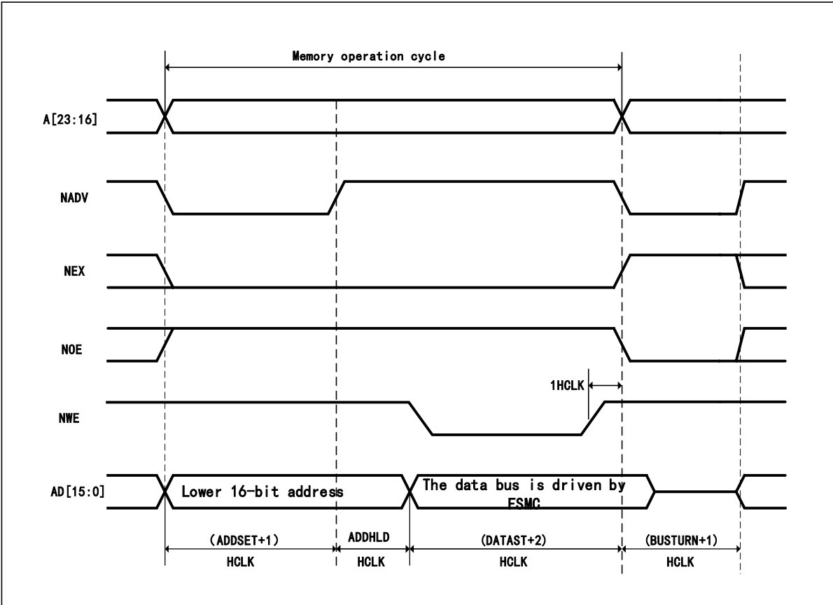
Figure 26-12 Mode D write operation (Multiplexed)
