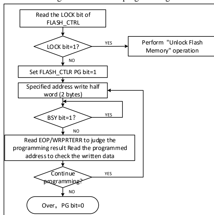
Figure 32-1 FLASH programming
