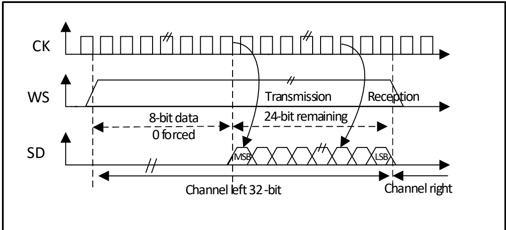
Figure 20-11 LSB-aligned 24-bit data, CPOL = 0
