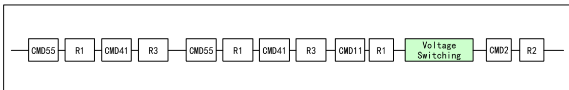
Figure28-13 Voltage switch sequence
