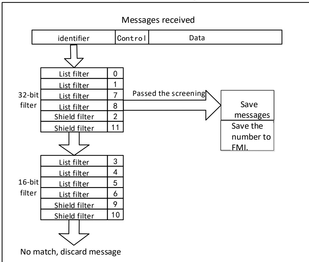
Figure 24-5 Filter example
