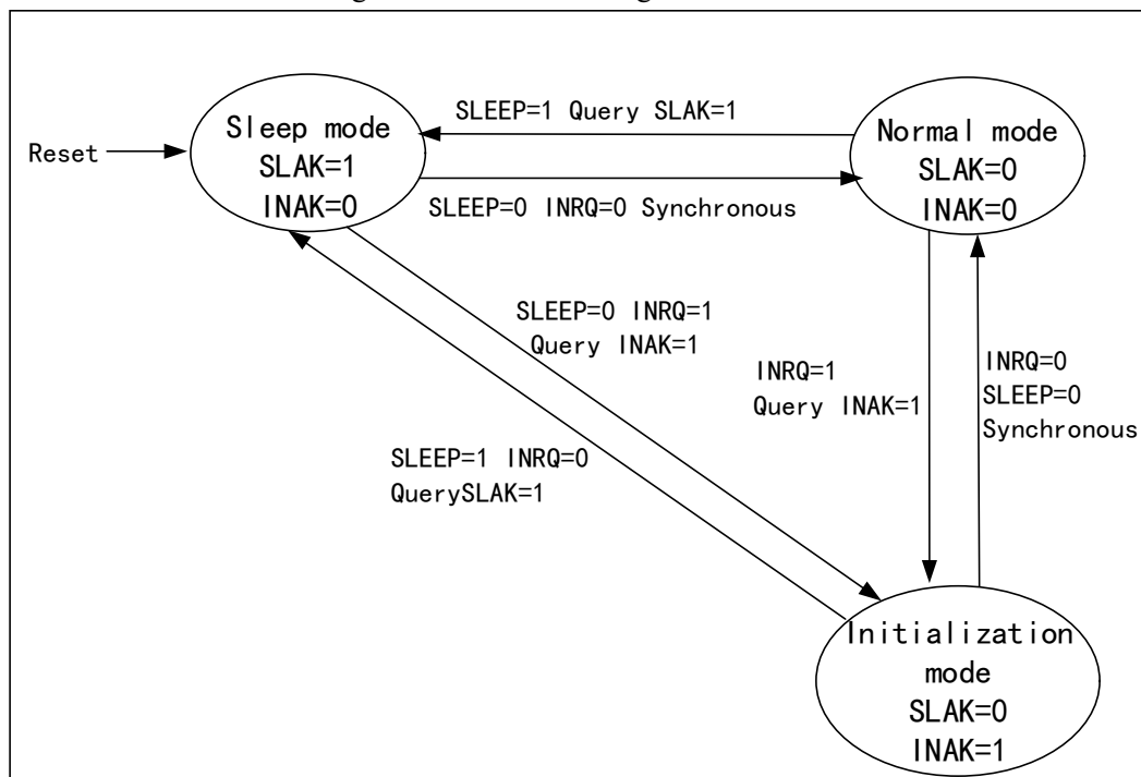
Figure 24-1 CAN working mode switch
