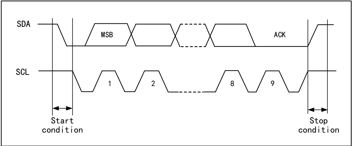
Figure 19-1 I2C timing diagram
