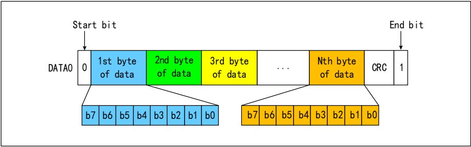
Figure 28-9 SD card single bus data transfer byte format
