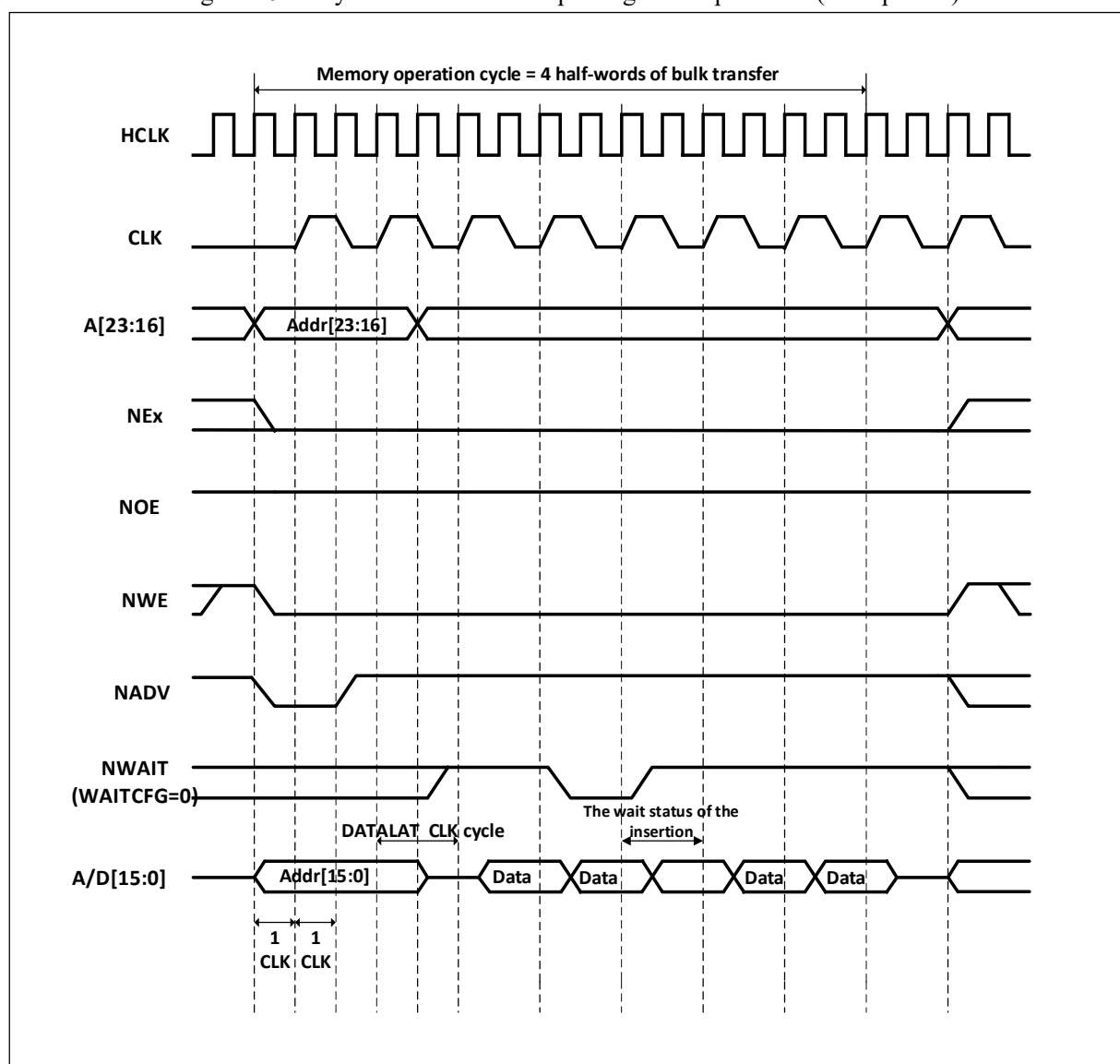
Figure 26-14 Synchronous bus multiplexing write operations (Multiplexed)
