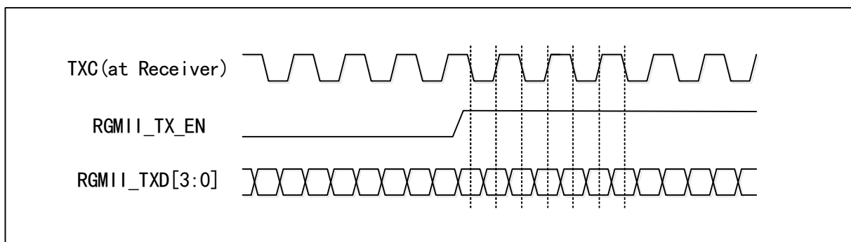
Figure 27-7 RGMII timing diagram
