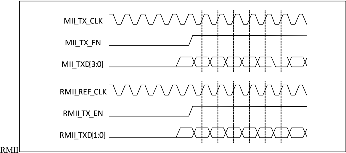
Figure 27-6 Timing diagram of MII and
