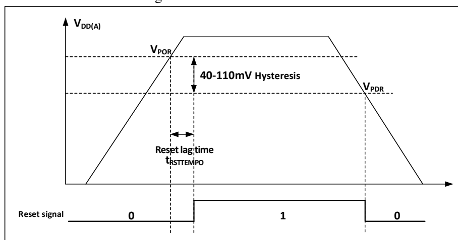
Figure 2-2 POR/PDR waveform
