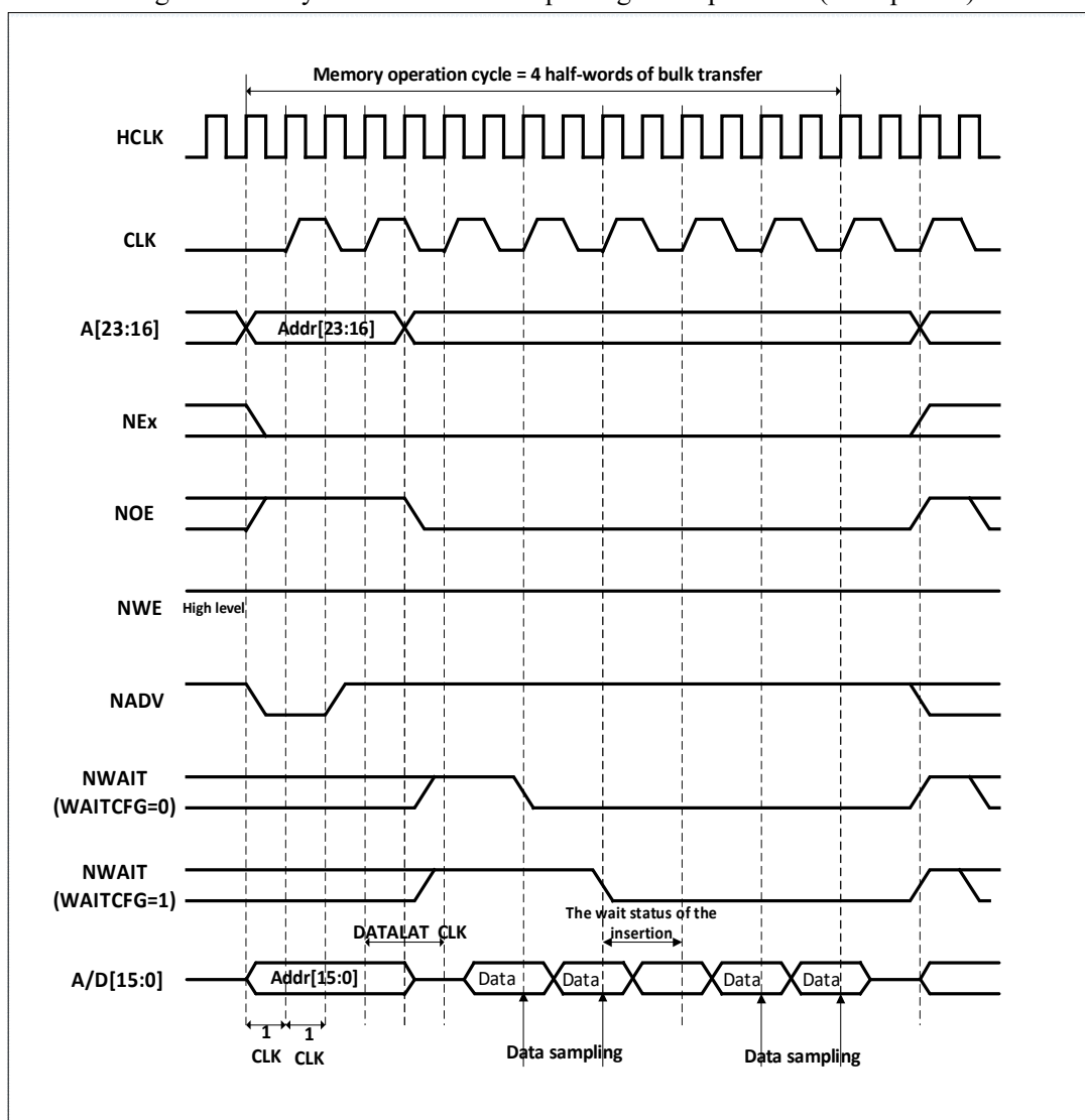
Figure 26-13 Synchronous bus multiplexing read operations (Multiplexed)
