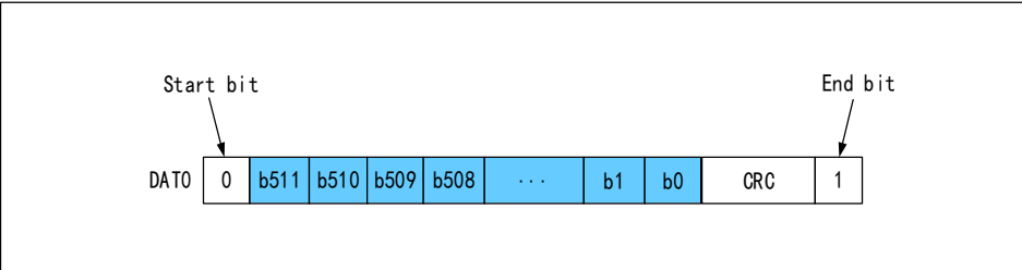
Figure 28-11 SD card single bus data transfer in a 512-bit word format
