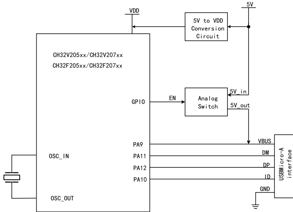
Figure 23-2 OTG Class A device connection
