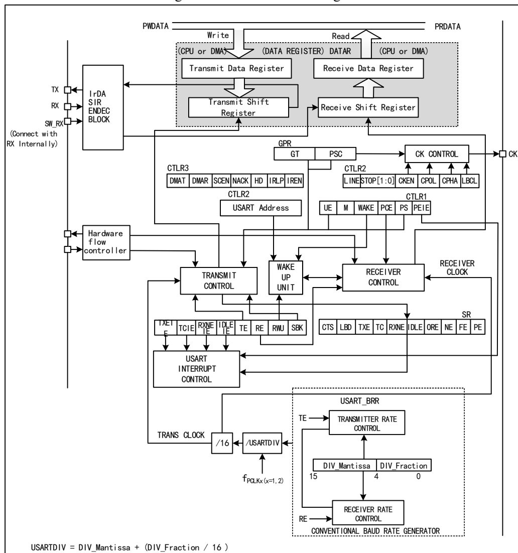
Figure 18-1 USART block diagram
