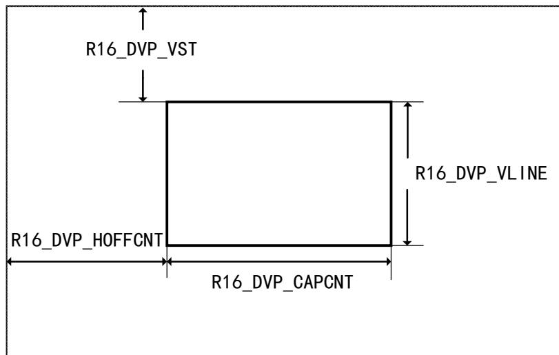
Figure 25-5 Crop window coordinates and size
