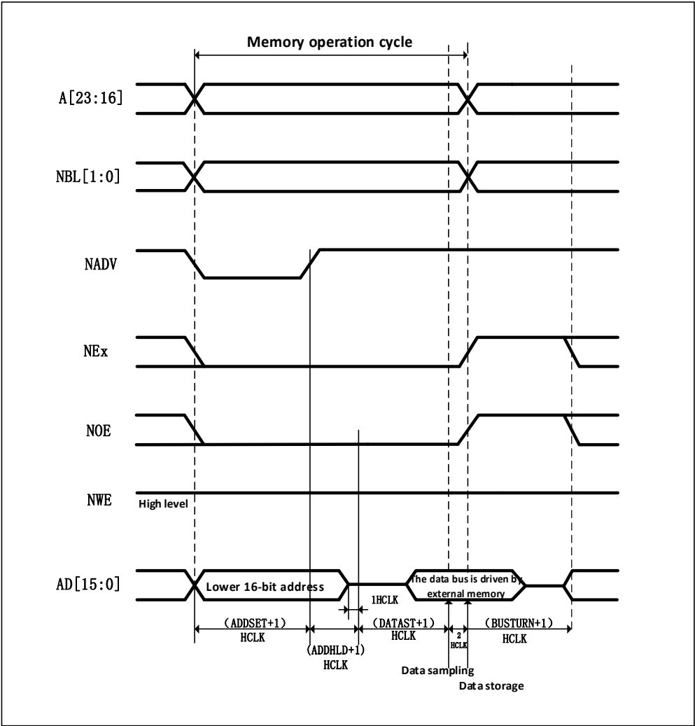
Figure 26-3 Mode 1 read operation (Multiplexed)
