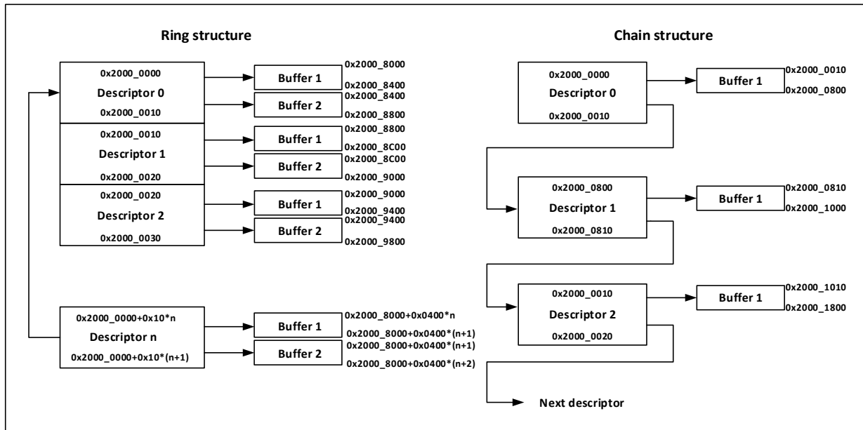
Figure 27-11 A buffer allocation scheme which describes the ring structure and the chain structure for reference when users allocate space.
