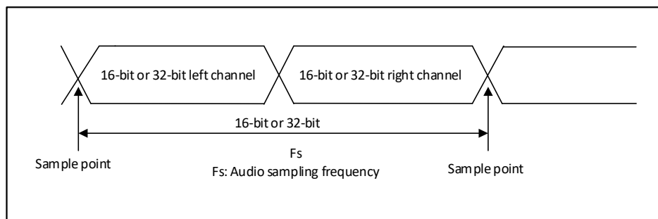
Figure 20-15 Audio sampling frequency definition
