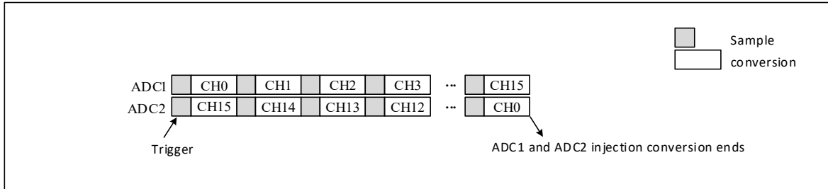
Figure 12-7 Regular simultaneous mode on 16 channels
