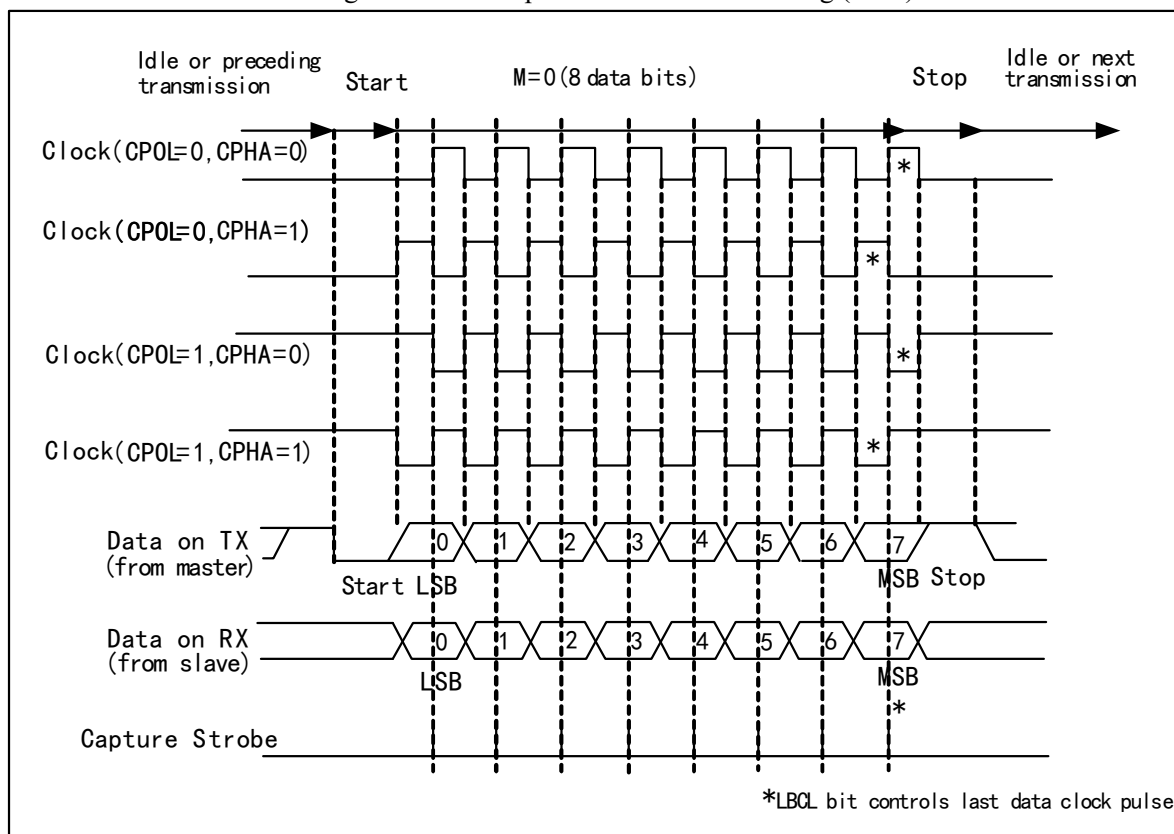
Figure 18-2 Example of USART clock timing (M=0)
