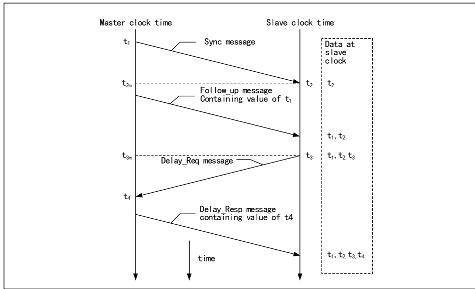
Figure 27-9 IEEE1588 PTP protocol synchronization message timing diagram
