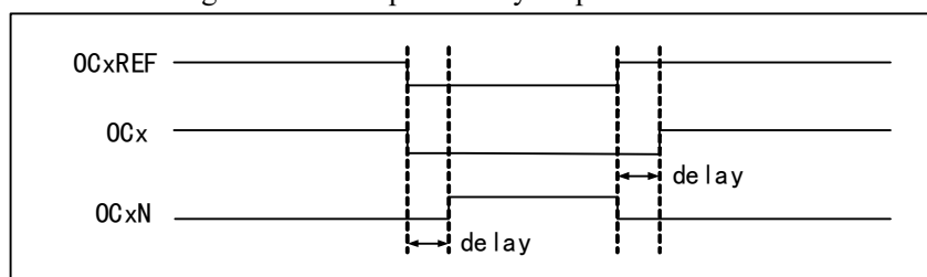
Figure 14-4 Complementary output and deadband
