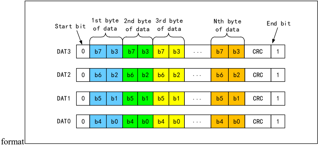
Figure 28-10 SD card 4 bus data transfer byte
