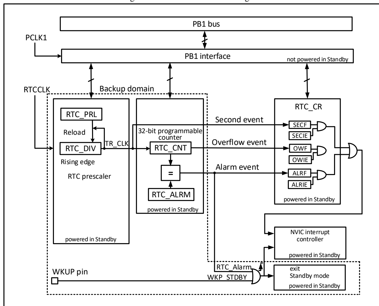
Figure 6-1 RTC structure block diagram
