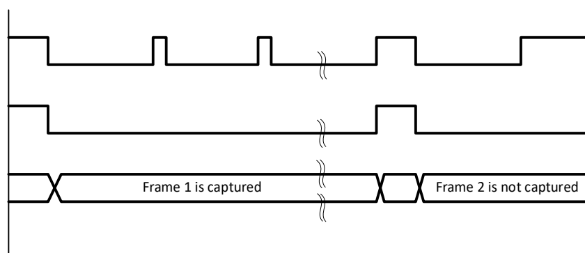
Figure 25-3 Single frame capture waveform in Snapshot mode
